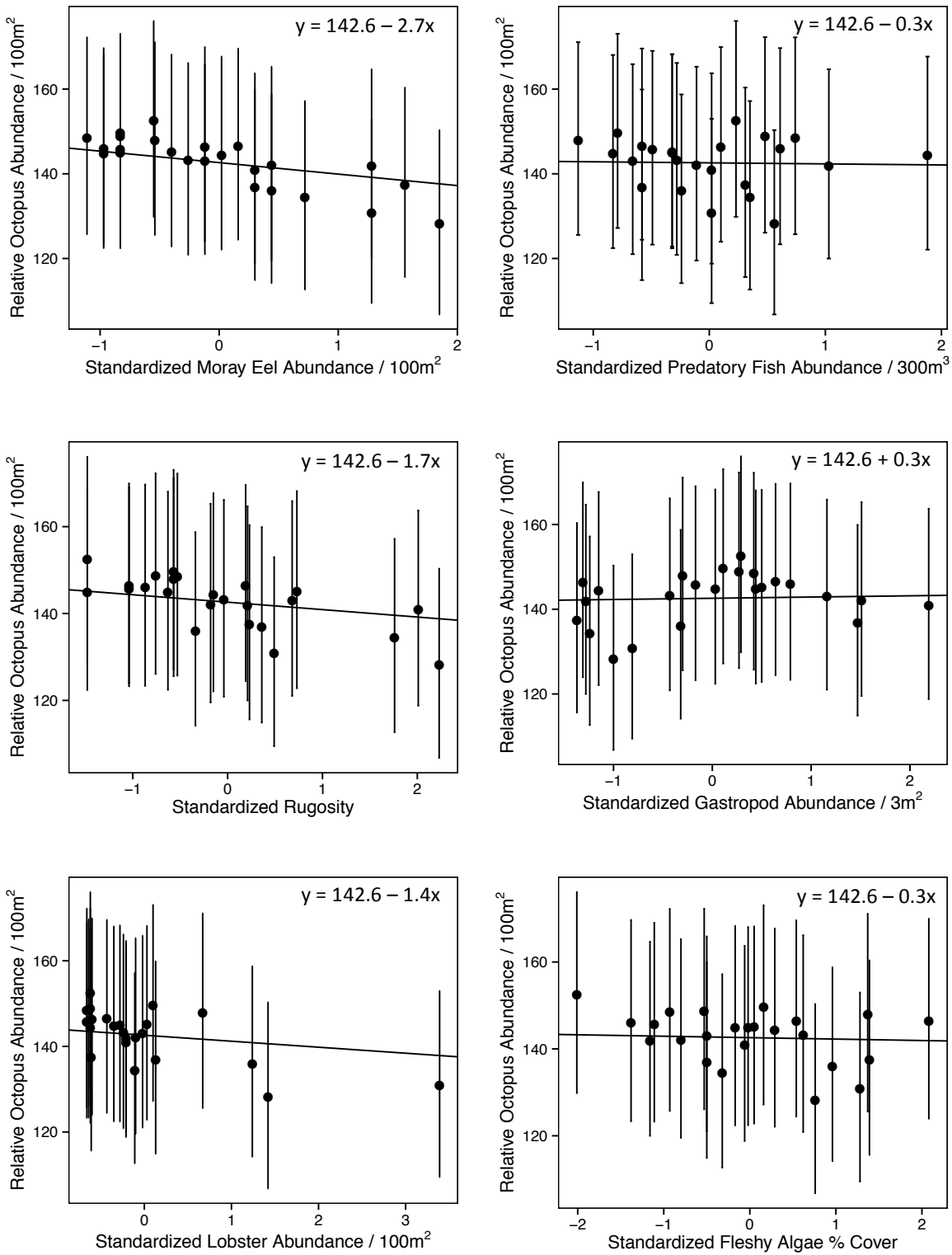
Figure 2.4. Mean relative octopus abundance (with 95% confidence intervals) against standardized (standard normal deviates) environmental covariates for 2013.
