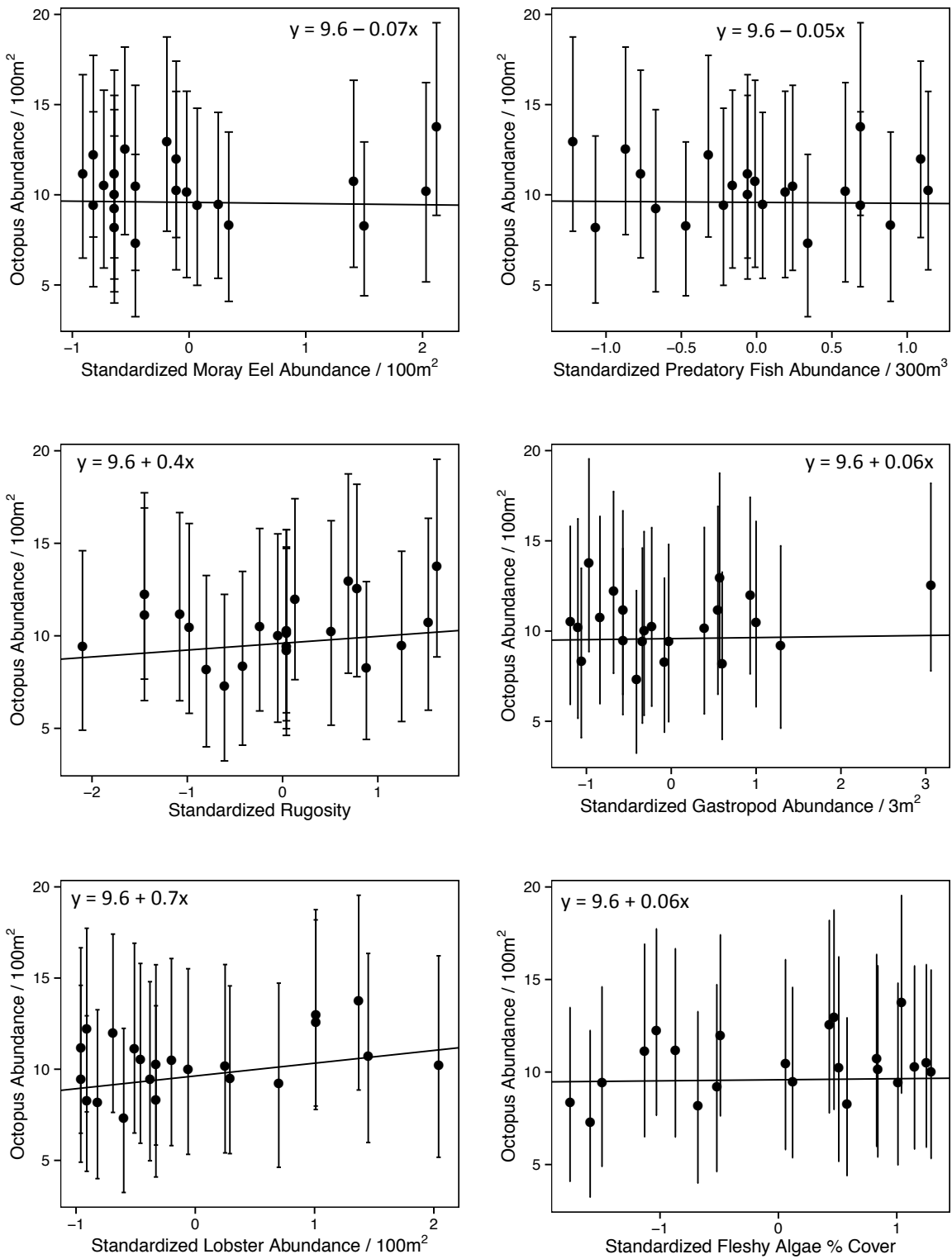
Figure 2.5. Mean octopus abundance (with 95% confidence intervals) against standardized (standard normal deviates) environmental covariates for 2014.
