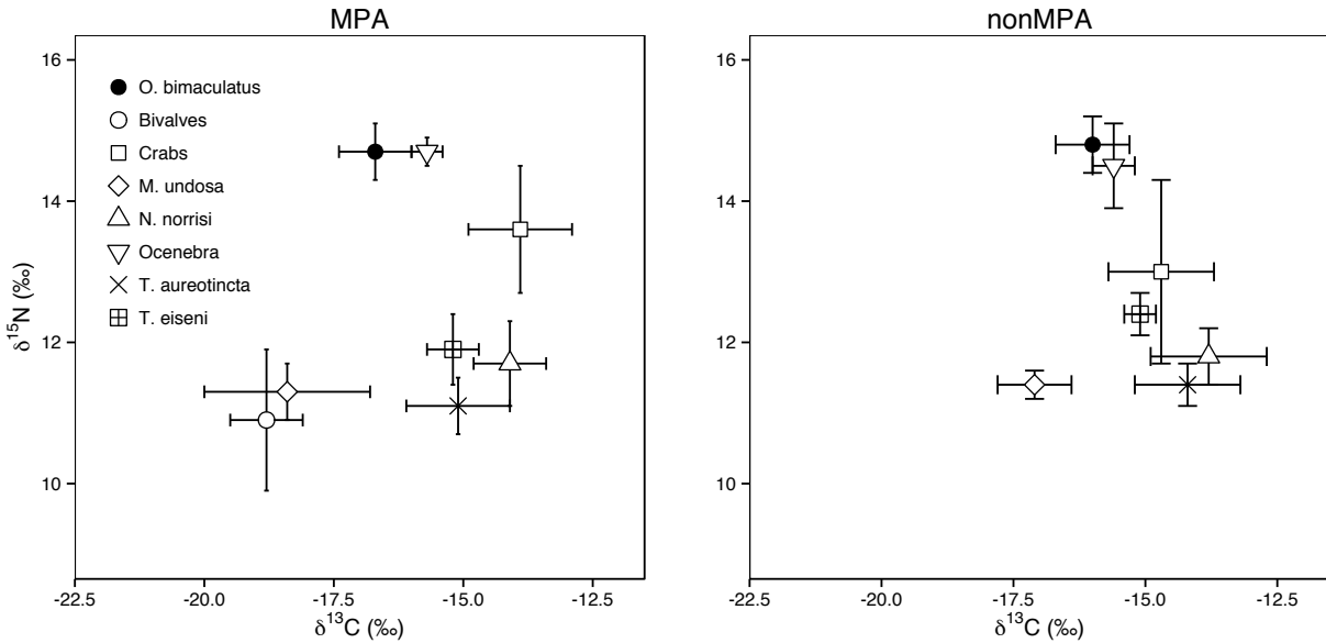
Figure 4.2. Graphic representation of mean ( \pm SD) \delta^{13}\text{C} vs. \delta^{15}\text{N} values of octopuses and their potential prey items, uncorrected for trophic fractionation, for all years combined. MPA graphs represent the full breadth of sampled prey items. NonMPA graphs do not include bivalves. The predatory snail, Ocenebra sp., has a similar \delta^{15}\text{N} value as the octopuses, consistent with predictions based on their carnivorous diet. Crabs have a \delta^{15}\text{N} value that fall in between the carnivores (octopuses and Ocenebra sp.) and algae-eating snails, consistent with predictions based on their omnivorous diet.
