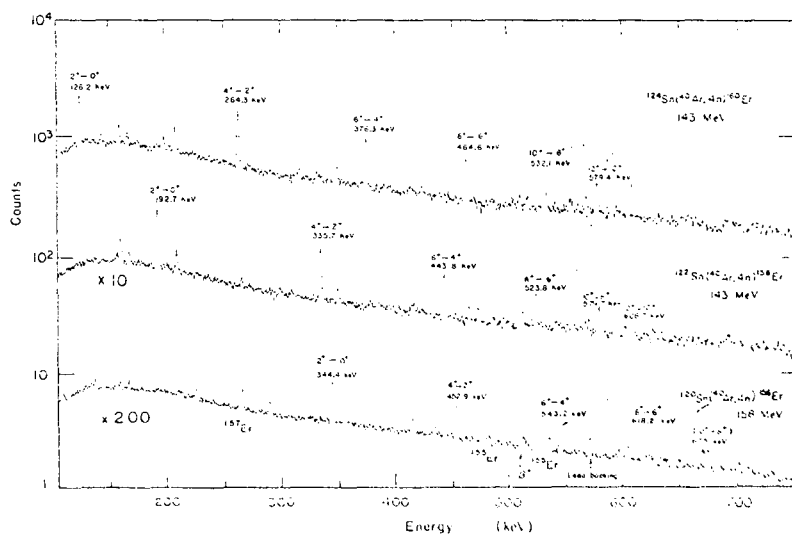
Fig. 1. Gamma-ray spectra following ^{40}\text{Ar}, 4n reactions, taken with a 6\text{ cm}^2 \times 0.8\text{ cm} deep \text{Ge}(\text{Li}) detector.
