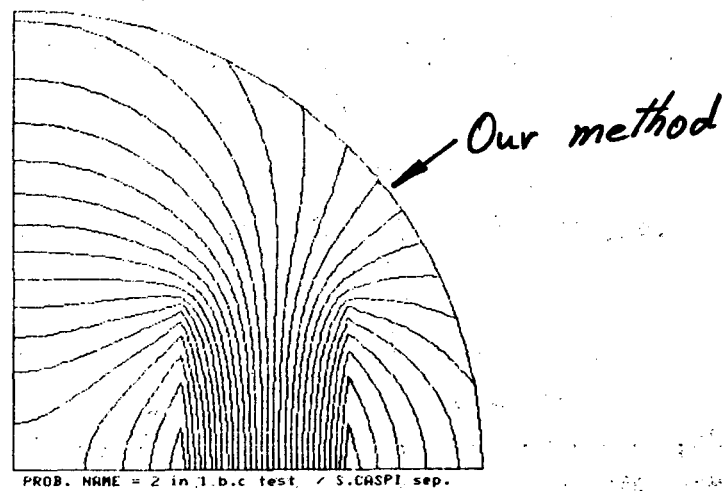
Fig. 5. Flux lines using the three different types of boundary conditions.
