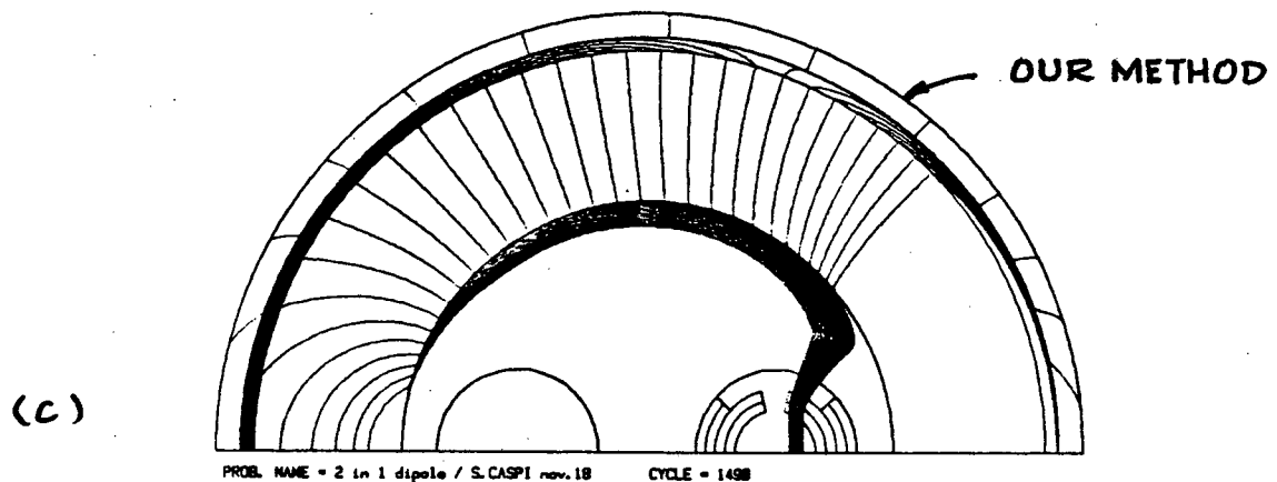
Fig. 7. A non-physical boundary condition can result in a non-physical solution. On top (case a) a Dirichlet condition results in flux lines circling the iron ring as if a net current flows through the dipole. In the center (case b) a Neumann condition results in flux lines which are prematurely returned to the iron ring. The correct flux lines are shown in the bottom (case c) using our method. It is however possible that when the boundary is farther removed from the iron ring, increasing the air and overall problem mesh size, both cases a and b can end up with reasonable flux lines.
