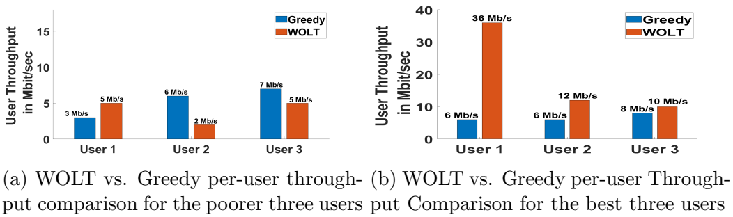
Figure 2.5: WOLT's Effects on Users' Throughputs
