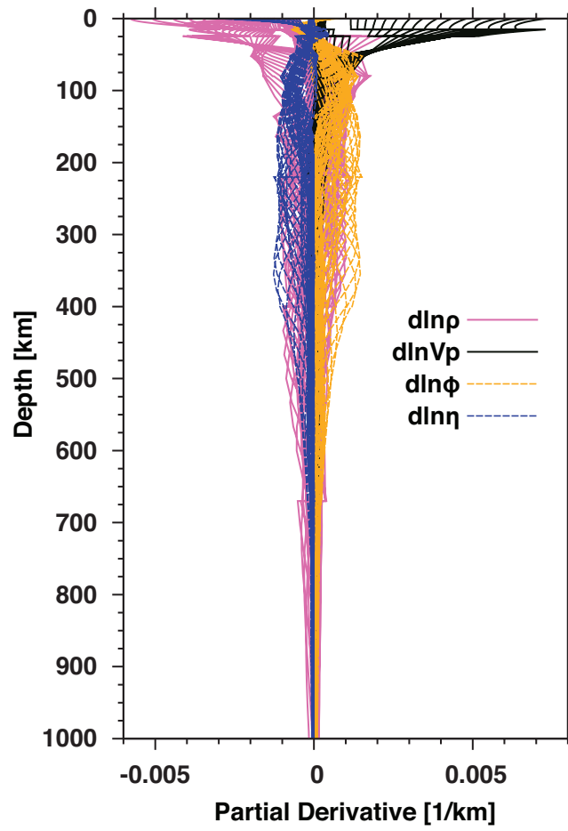
Figure 3. Sensitivity Kernels for Rayleigh and Love Wave fundamental modes and first two overtones calculated used in this study. The kernels were calculated for d \ln V_p , d \ln \phi , d \ln \eta , and d \ln \rho .
