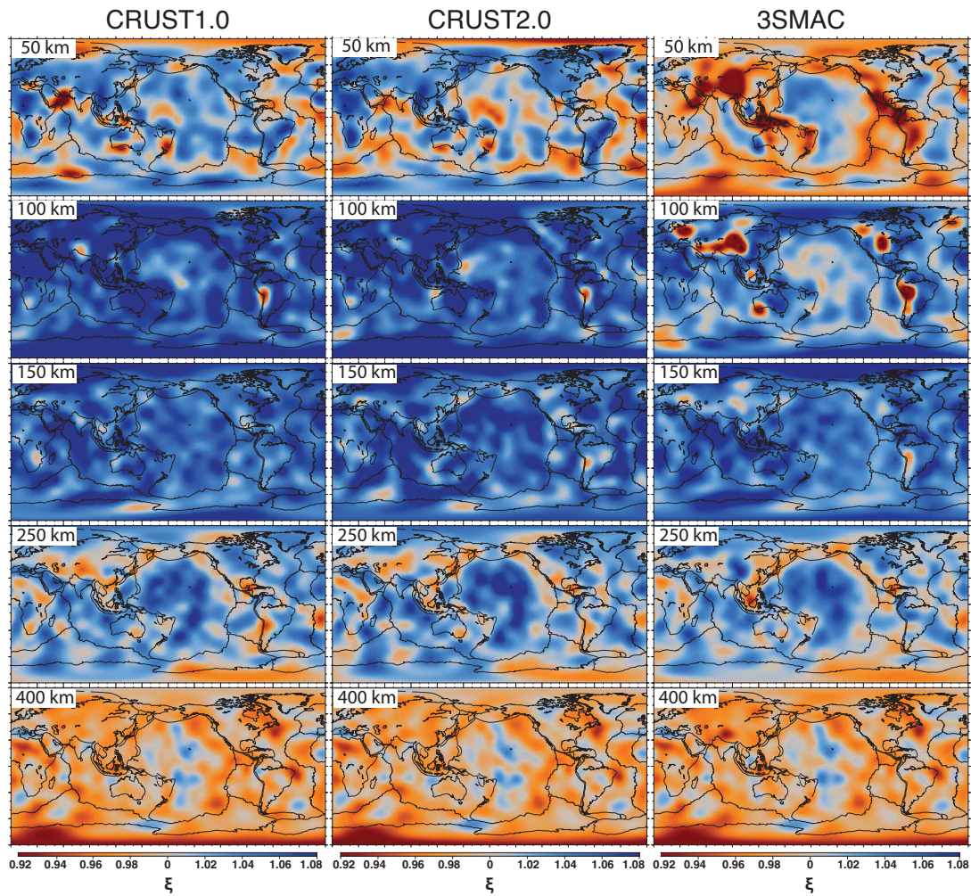
Figure 9. Radial anisotropy at 50 km, 100 km, 150 km, 250 km, and 400 km obtained using, from left to right, CRUST1.0, CRUST2.0, and 3SMAC. \xi = 1 corresponds to an isotropic mantle model. \xi > 0 corresponds to V_{SH} > V_{SV} .
