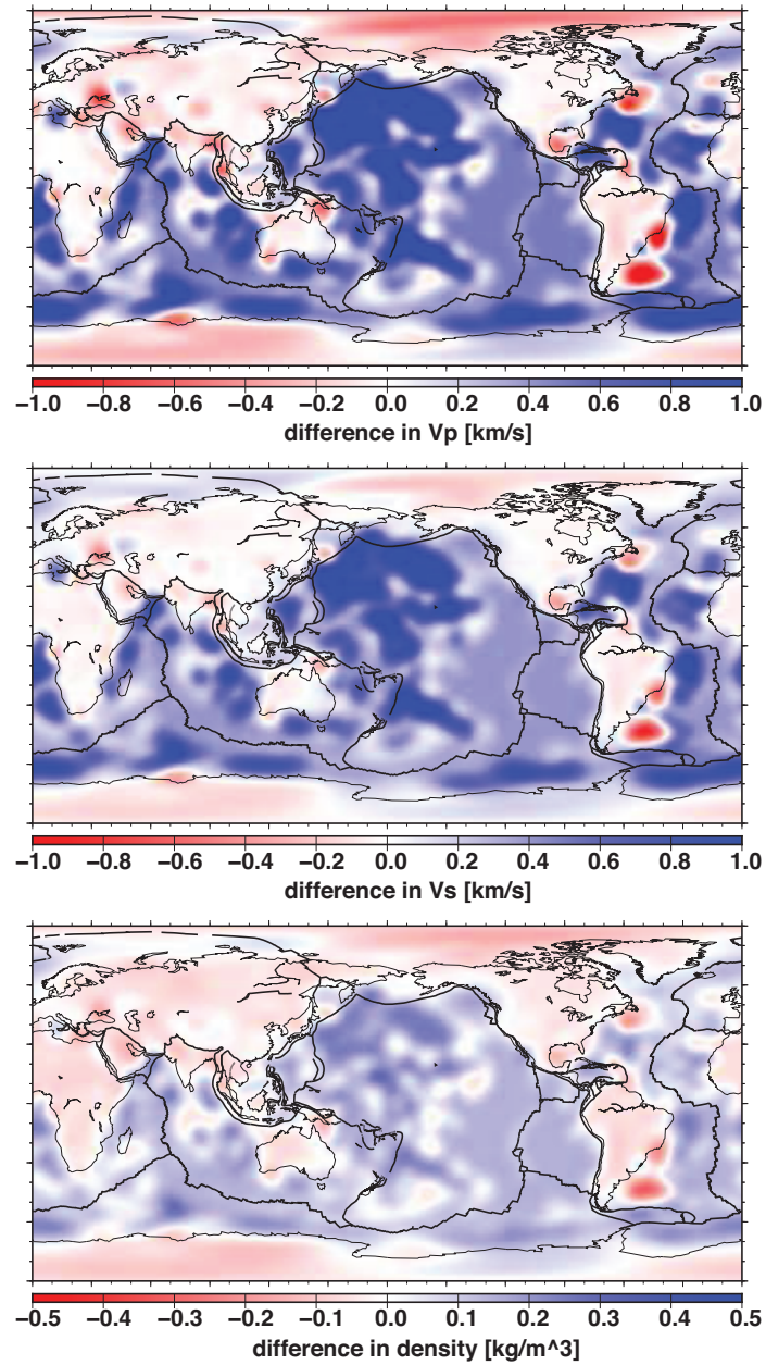
Figure 5. Example of difference in velocities and density between CRUST1.0 and CRUST2.0 at 7 km depth.
