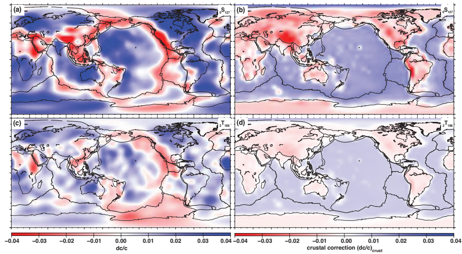
Figure 1. (a): Fundamental mode Rayleigh wave phase velocity maps at 78 s (Visser et al. 2008a) and (b) corresponding crustal correction using CRUST2.0 (Bassin et al. 2000); (c): Second overtone Love wave phase velocity maps at 40 s and (d) corresponding crustal correction.
