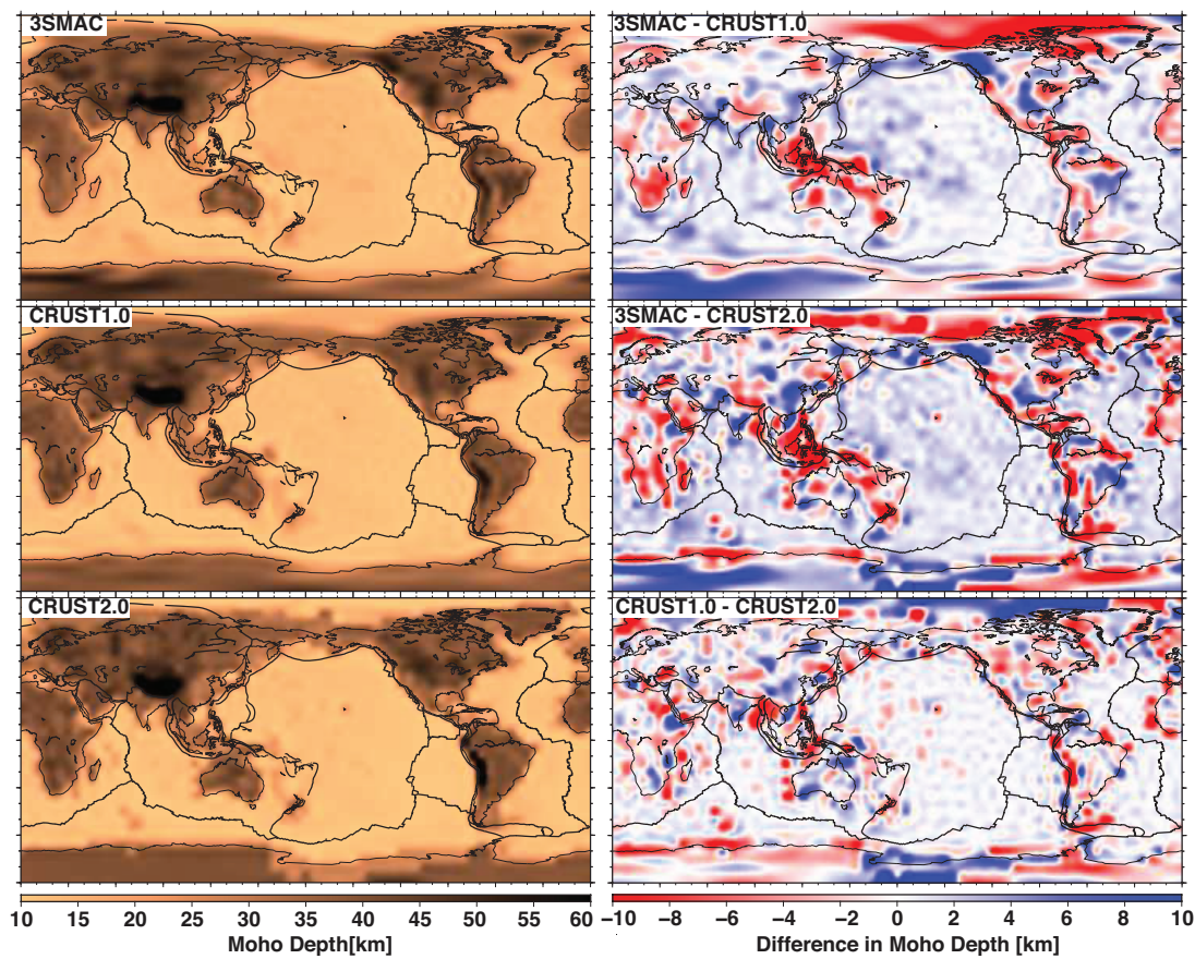
Figure 4. Moho depths (left) for 3SMAC, CRUST1.0 and CRUST2.0 and differences (right) between each pair of models.
