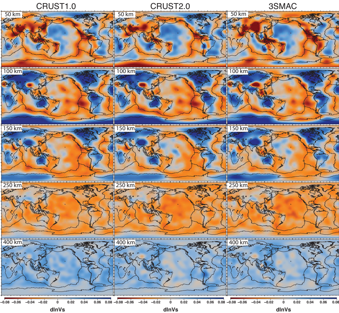
Figure 8. Shear velocity perturbations with respect to PREM at 50 km, 100 km, 150 km, 250 km, and 400 km obtained using, from left to right, CRUST1.0, CRUST2.0, and 3SMAC.
