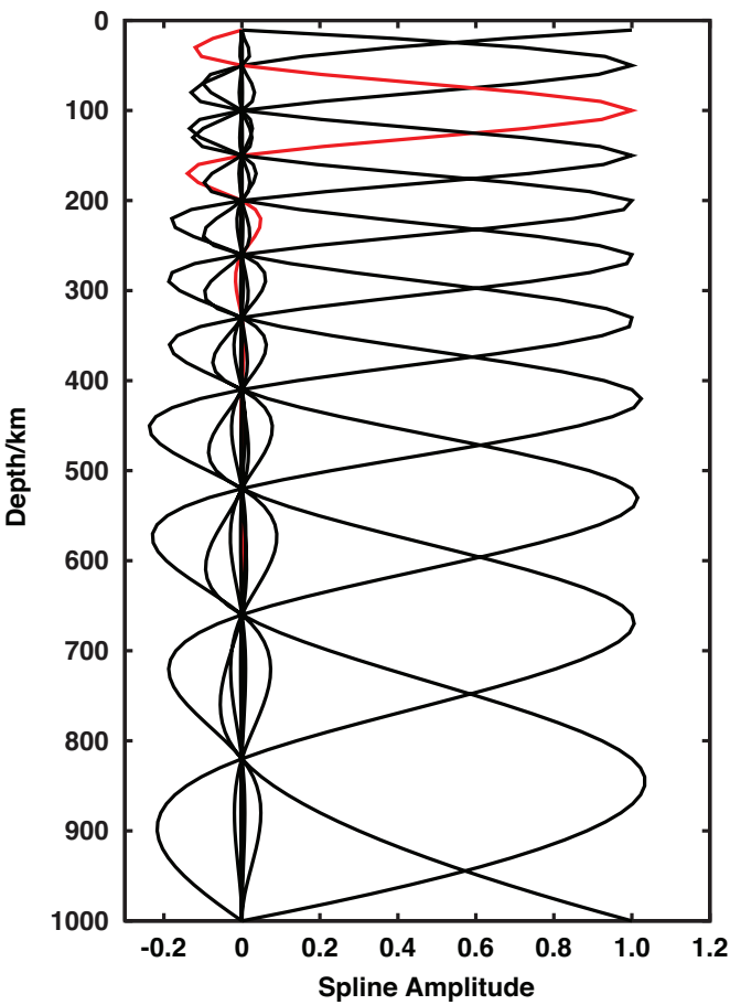
Figure 6. Spline functions used for the depth parameterization. The interval increases with depth to account for the decrease in sensitivity. The red curve highlights the spline that peaks at 100 km depth.
