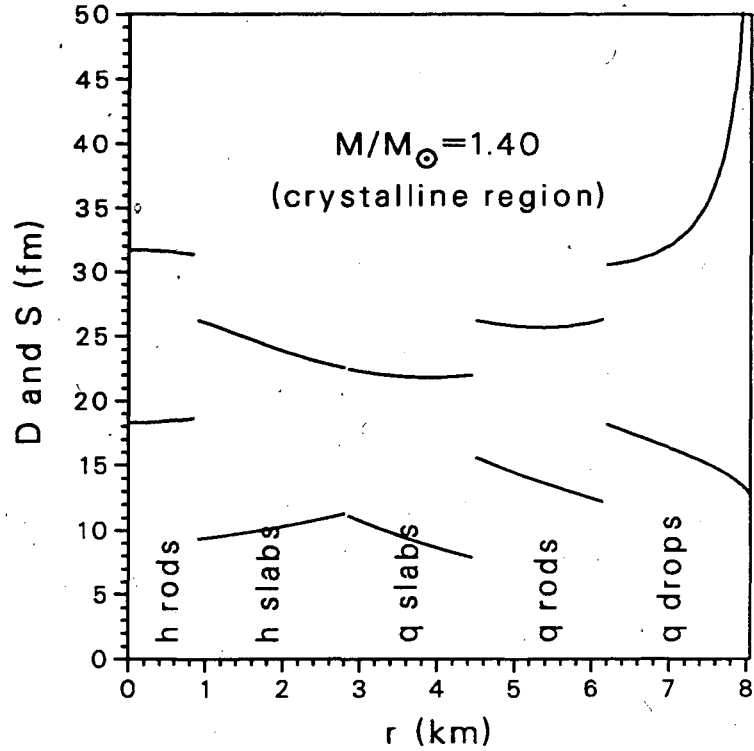
Figure 2: Similar to previous figure but for slightly less massive star. Mixed crystalline phase now extends to star's center. Radius is 12.3 km.
