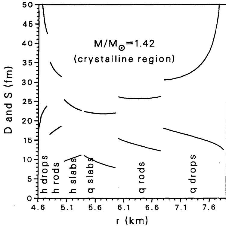
Figure 1: Crystalline mixed region in a neutron star showing the diameter D (lower curves) and spacing S (upper curves) of indicated geometric structures as a function of radial Schwarzschild coordinate. Region internal to 4.6 km is pure quark matter. Notation ‘h drops’ denotes hadronic drops immersed in quark matter, and so on. Stellar radius is 10.7 km.
