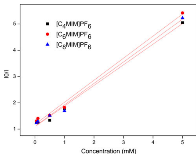
Fig. 7 The Stern-Volmer plot for BPA in [C_n\text{MIM}]\text{PF}_6
