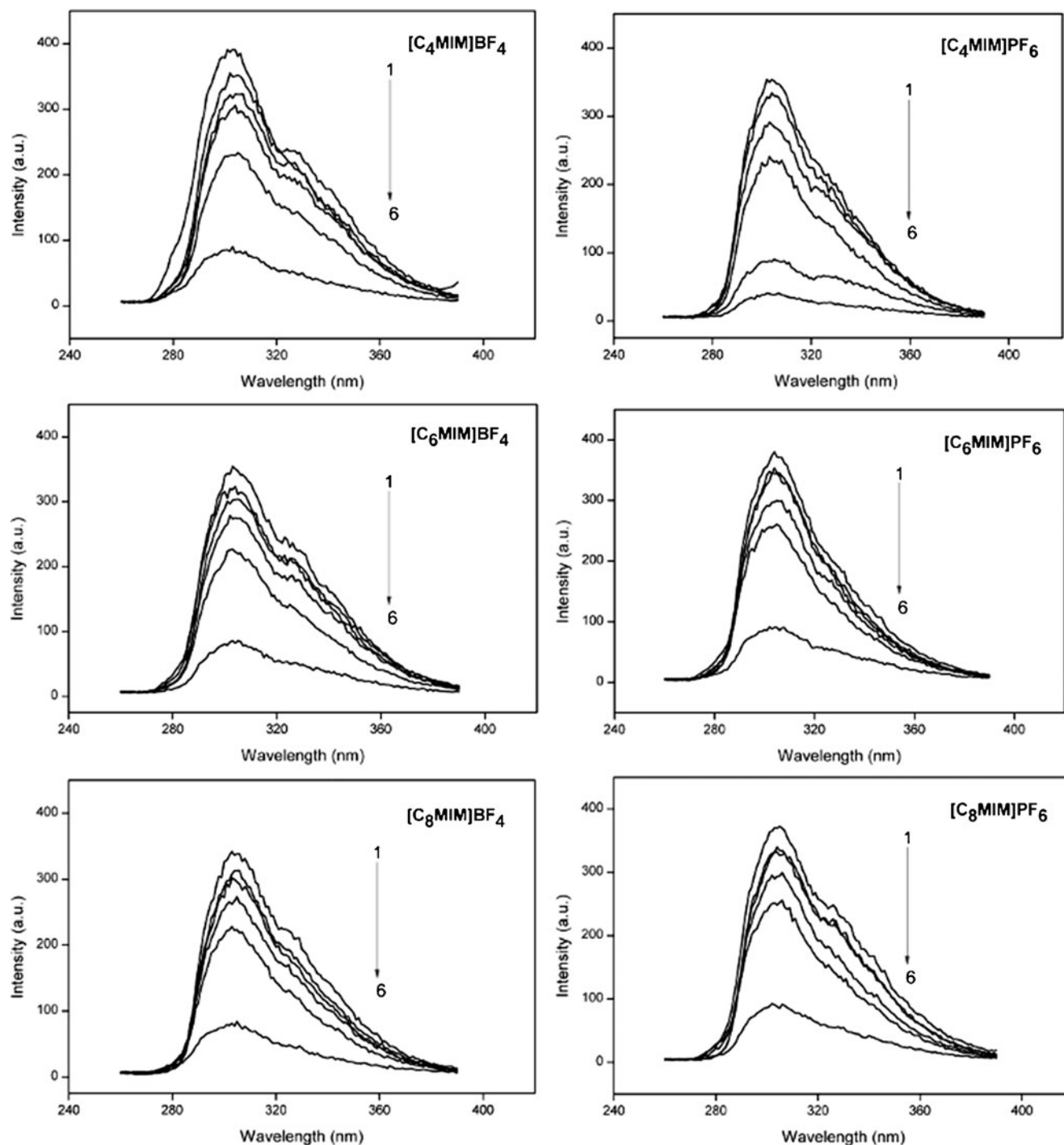
Fig. 1 The fluorescence emission spectra of BPA in acetonitrile and RTIL-acetonitrile systems. Note: 1–6 indicates 0, 0.05, 0.1, 0.5, 1.0, 5.0 mM RTILs
