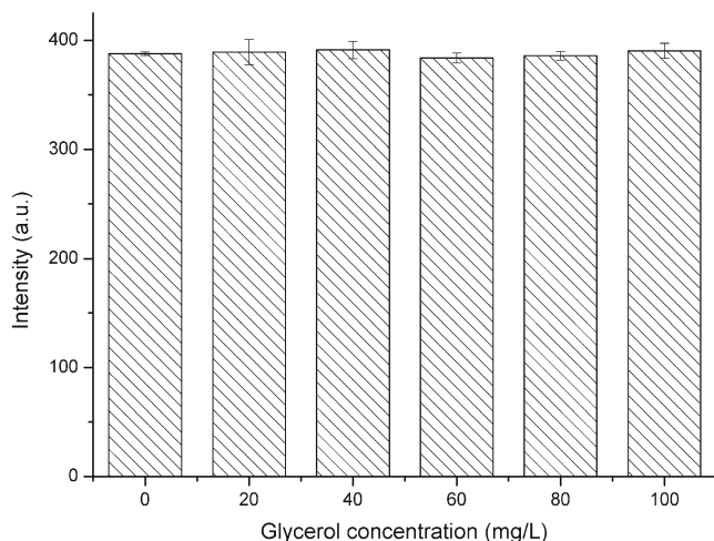
Fig. 2 The effect of solvent viscosity on the FIs of BPA
