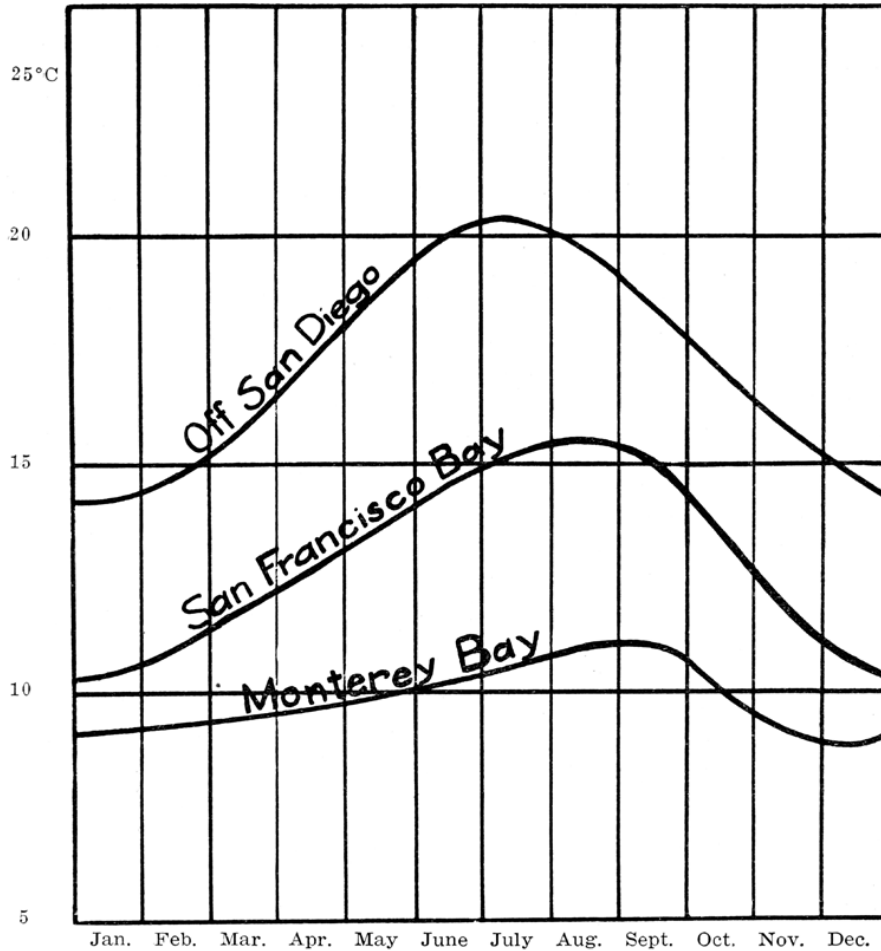
PLATE I. Smoothed curves showing the variation in temperature throughout the year at three points along the California coast.
