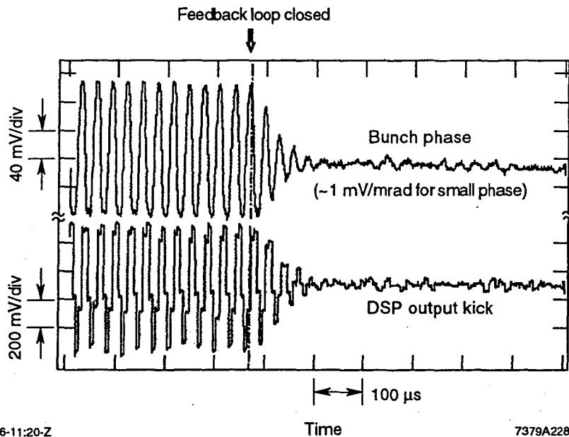
Fig. 3. Bunch phase deviation (upper trace) and DSP output (lower trace) for SPEAR measurements. The bunch is excited with the feedback loop open and then the loop is closed (dashed line), after which the bunch recovers quickly to baseline.
