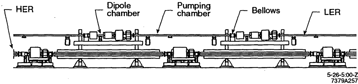
Fig. 2. Side view of HER and LER FODO cells showing magnet layout.
