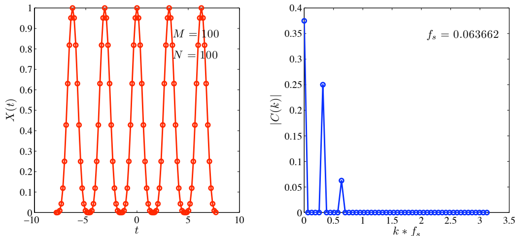
Figure B.9: Fourier spectrum of the function \cos^4(t) with a longer sample period T than in Fig. B.8. Again, there are three nonzero frequency components at f = 0, 1/\pi and 2/\pi .
