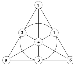
Figure 2.1: The Fano plane is an example of a projective plane.
