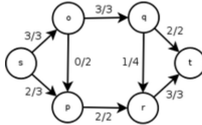
Figure 3.1: A transportation network with flow and capacity denoted f/c .
