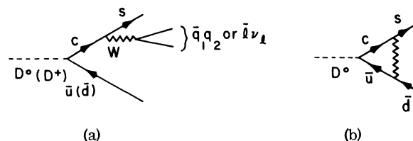
FIG. 1. Graphs contributing to D -meson decays. (a) The "spectator" graph that contributes to the nonleptonic and semileptonic decays of both the charged and the neutral D mesons. (b) This contributes to the decays of the D^0 ( \bar{D}^0 ) only. See Ref. 3.
