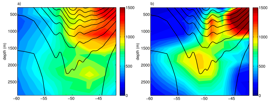
FIG. 9. Along-stream averages of diffusivities as a function of depth and lat averaged over the bin for each streamline bin. (a) Lagrangian and (b) Eulerian diffusivities ( \text{m}^2 \text{s}^{-1} ). Contours are Eulerian mean velocity averaged along the streamline bins.
