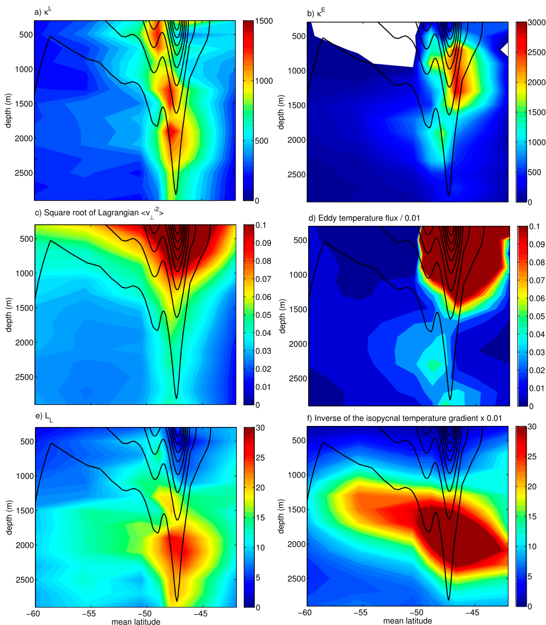
FIG. 10. Average over 120^{\circ} – 145^{\circ} E, the western half of lon bin 4 from Fig. 6, corresponding to an average over two overlapping bins. (a) Lagrangian and (b) Eulerian diffusivities ( \text{m}^2 \text{s}^{-1} ), (c) Lagrangian \sqrt{\langle v_{\perp}^2 \rangle} ( \text{m s}^{-1} ), (d) Eulerian eddy temperature flux divided by 0.01 ( \text{m s}^{-1} \text{C}^{-1} ), (e) Lagrangian eddy integral scale (km), and (f) Eulerian reciprocal of the isopycnal temperature gradient times 0.01 ( \text{m}^{\circ}\text{C}^{-1} ). The factor 0.01 was chosen to be able to better compare the vertical structure of Eulerian and Lagrangian quantities.
