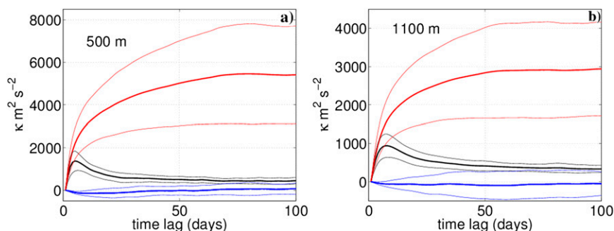
FIG. 3. Lagrangian diffusivity tensor components as a function of time lag in along-streamline average for a depth of (a) 500 and (b) 1100 m and mean lat 52°S: black is \kappa_{\perp} , magenta is \kappa_{\parallel} , and blue is \kappa_{\perp\parallel} . Also shown in thin lines is the std dev of the along-streamline average.
