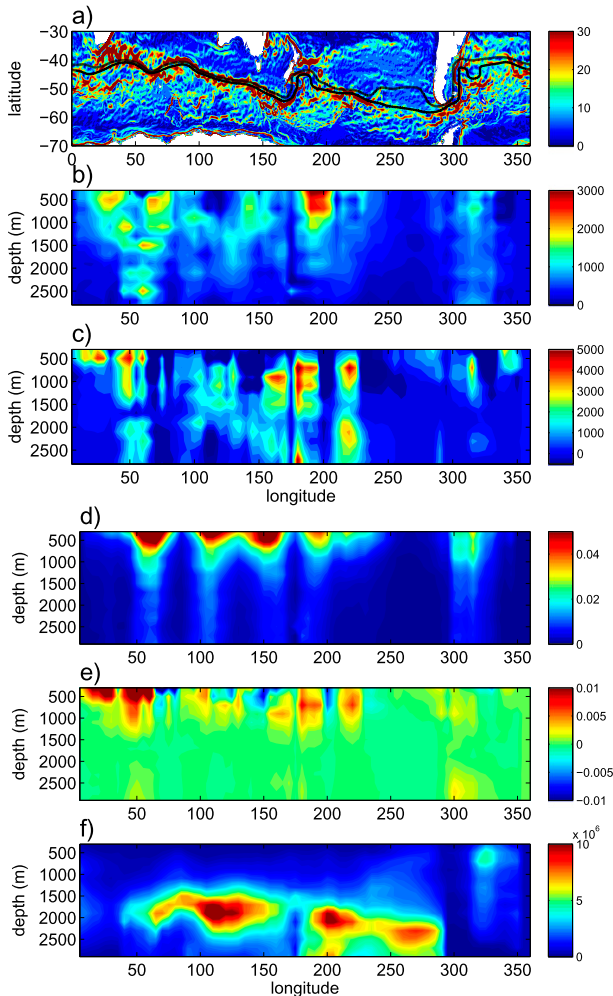
FIG. 12. (a) Along-streamline variation of quantities for the streamline bin shown together with the Eulerian mean velocity (color). (b) Lagrangian and (c) Eulerian diffusivities ( \text{m}^2 \text{s}^{-1} ). (d) Lagrangian \langle u'^2 \rangle ( \text{m}^2 \text{s}^{-2} ). (e) Eulerian cross-temperature contours eddy heat flux ( ^\circ\text{C m}^{-1} \text{s}^{-1} ). (f) Reciprocal of Eulerian isopycnal temperature gradient ( ^\circ\text{C m}^{-1} ).
