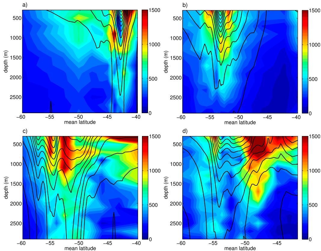
FIG. 7. Lagrangian cross-stream diffusivity as a function of depth and latitude ( \text{m}^2\text{s}^{-1} ). Bins (a) 3, (b) 6, (c) 8, and (d) 5 from Fig. 6. Contours are Eulerian mean velocity averaged along the streamline bins.
