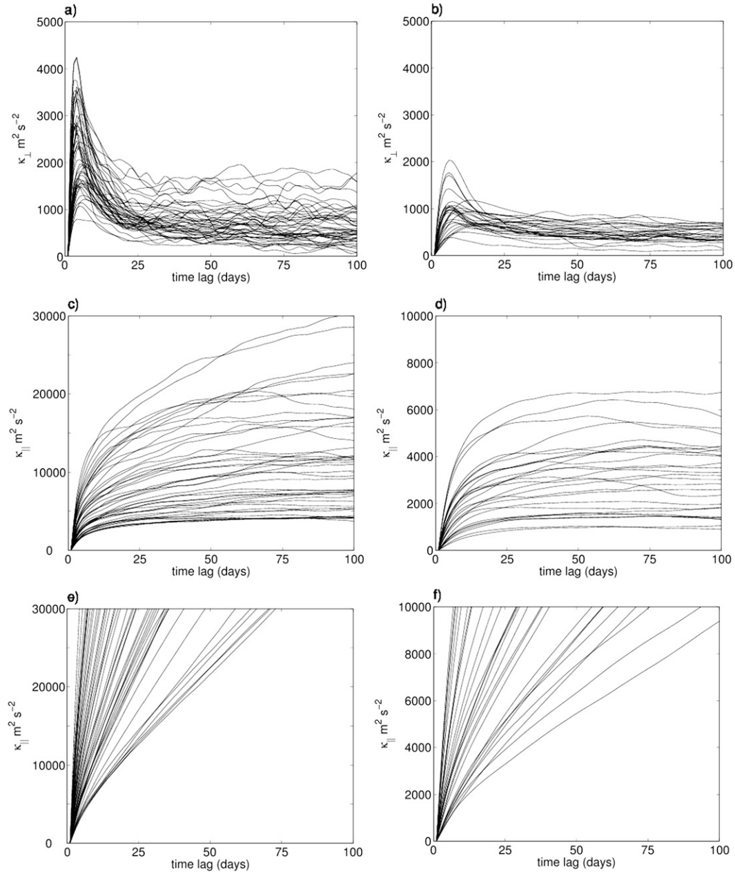
FIG. 2. Cross-stream diffusivity as a function of time lag in the core of the ACC for bins at (a) 300 and (b) 1500 m. (c),(d) As in (a),(b), but for along-stream diffusivity. (e),(f) Along-stream diffusivity as in (c),(d), but without subtraction of the Eulerian mean. Note the different scales on the y axes.
