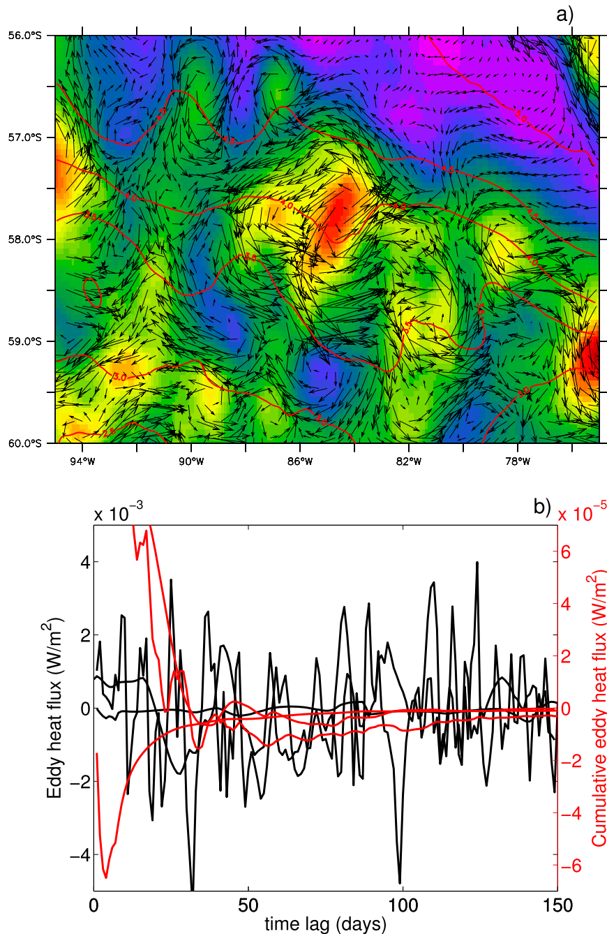
FIG. 8. (a) Horizontal eddy flux (vectors; \text{W m}^{-2} ), eddy variance \overline{\theta'^2} (color; ^{\circ}\text{C}^2 ), and \overline{\theta} (contours; ^{\circ}\text{C} ) for a region west of the Drake Passage. (b) Cross-stream eddy heat flux along three trajectories (black, left axis; \text{W m}^{-2} ) and associated cumulative mean cross-stream heat flux averaged along each trajectory (red, right axis; \text{W m}^{-2} ).
