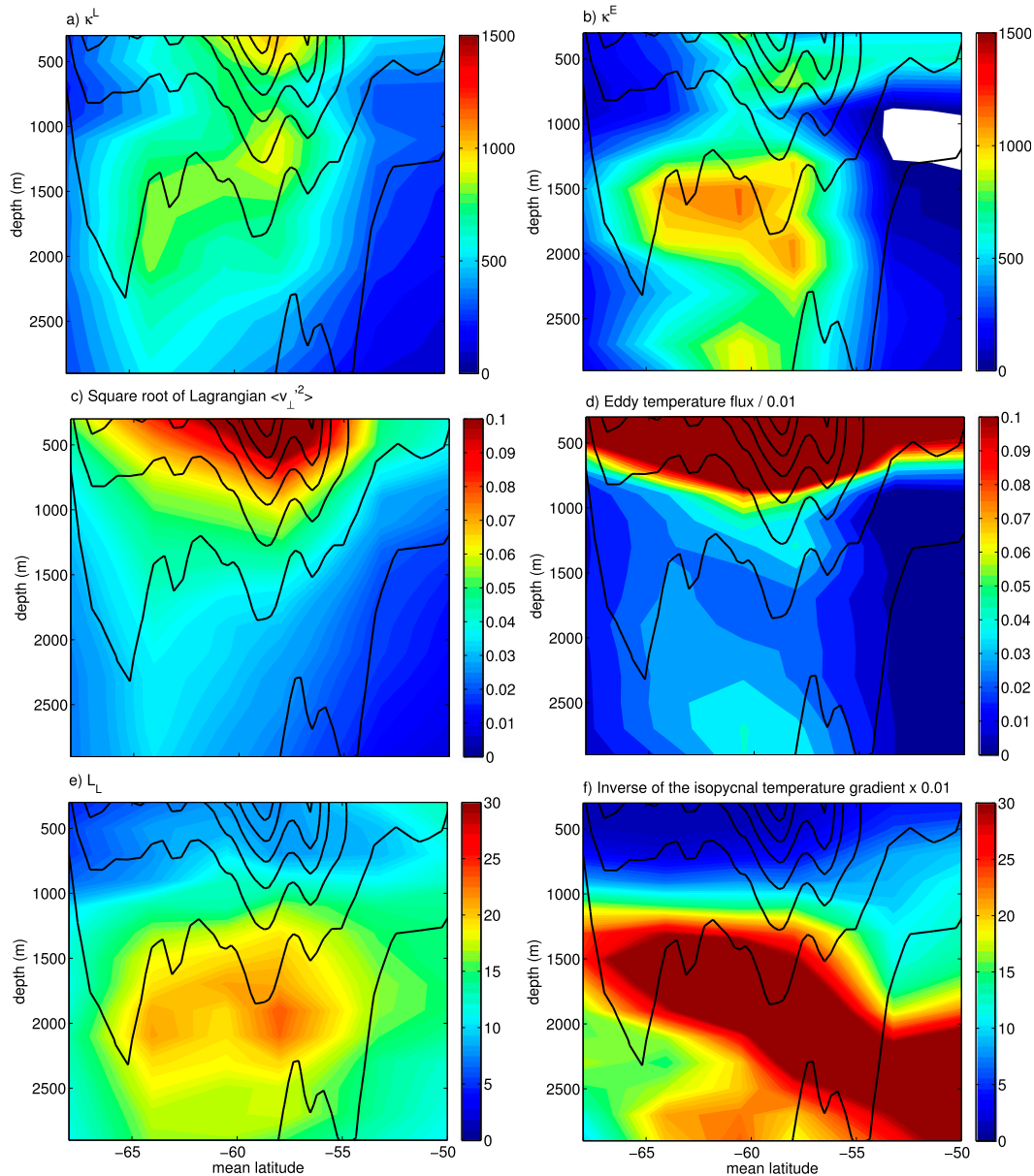
FIG. 11. Average over 240°–280°E, lon bin 7 from Fig. 6, corresponding to an average over five overlapping bins in lon. (a) Lagrangian and (b) Eulerian diffusivities ( \text{m}^2 \text{s}^{-1} ), (c) Lagrangian \sqrt{\langle v_{\perp}^2 \rangle} ( \text{m s}^{-2} ), (d) Eulerian eddy heat flux divided by 0.01 ( \text{m s}^{-1} \text{C}^{-1} ), (e) Lagrangian eddy integral scale (km), and (f) Eulerian reciprocal of the isopycnal temperature gradient times 0.01 ( \text{m}^{\circ}\text{C}^{-1} ). The factor 0.01 was chosen to be able to better compare the vertical structure of Eulerian and Lagrangian quantities.
