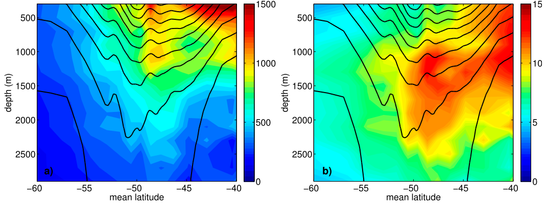
FIG. 5. (a) Along-streamline average of Lagrangian diffusivity ( \text{m}^2 \text{s}^{-1} ). The profile around 50^\circ\text{S} corresponds to the red line in Fig. 4. (b) Along-streamline average of Lagrangian integral length scale (km). Contours are Eulerian-mean velocity averaged along the streamline bins with a contour interval of 2 \text{ cm s}^{-1} .
