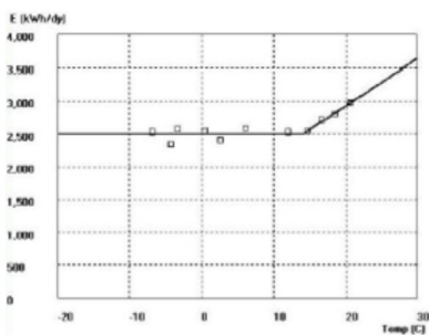
Monthly Regression R^2 = 0.89
