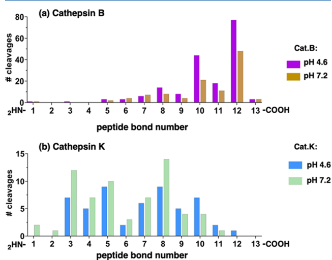
Figure 2. Cleavage profiling of cathepsin B DPCP and endopeptidase activities by MSP-MS conducted at acidic pH 4.6 and neutral pH 7.2. (a) Cathepsin B MSP-MS under acidic and neutral pH conditions demonstrates major DPCP activity. Cathepsin B was subjected to MSP-MS analysis of exopeptidase and endopeptidase cleavage sites at pH 4.6 and pH 7.2 (using four technical replicates). The number of cleavages at peptide bonds #1–13 of the diverse library of 228 peptides after incubation for 15 min was determined as described in the methods. At pH 4.6, 179 cleavages were assessed in the plotted graph for the number of cleavages at each peptide bond location. At pH 7.2, 109 cleavages of the peptide library are graphed similarly. This MSP-MS experiment was conducted two times. (b) Cathepsin K MSP-MS under acidic and neutral pH conditions demonstrates major endopeptidase activity. Cathepsin K was subjected to MSP-MS analysis at pH 4.6 and pH 7.2. The number of cleavages at each of the peptide bonds #1–13 of the peptide library generated after 15 min incubation was determined as described in the methods using four technical replicates.
