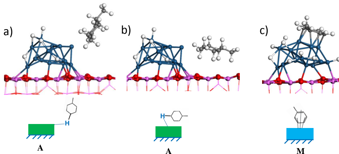
Figure 5. Adsorption of (A) methyl-cyclohexane a) in the perpendicular mode, b) in the flat mode, and c) of (M) toluene on \text{Pt}_{13}\text{H}_6/\gamma\text{-Al}_2\text{O}_3 . Color legend: aluminum (pink balls), oxygen (red balls), platinum (dark blue balls), carbon (dark grey balls), hydrogen (white balls)
