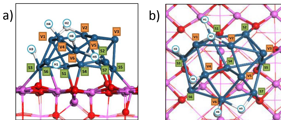
Figure 1. Molecular structure of the starting model of \text{Pt}_{13}/\gamma\text{-Al}_2\text{O}_3 (100) with 6 adsorbed hydrogen atoms. a) side view, b) top view. Pt atoms labelled with letter “S” are located at the alumina surface, Pt atoms labelled with letter “V” are in contact with vacuum. Color legend: aluminum (pink balls), oxygen (red balls), platinum (dark blue balls), hydrogen (white balls)
