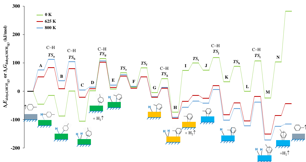
Figure 4. Free energy profile (PBE-dDsC level) for methyl-cyclohexane dehydrogenation over \text{Pt}_{13}\text{H}_6/\gamma\text{-Al}_2\text{O}_3 at 0 K, 625 K and 800 K. Each colored box represents the cluster with 6 H atoms and various colors correspond to different cluster morphologies (also highlighted in Figures 5 and 6 with the same color coding).
