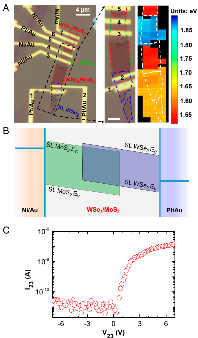
Fig. 4. Electrical transport across the \text{WSe}_2/\text{MoS}_2 hetero-interface. (A) Optical microscope image of a device encompassing single-layer \text{WSe}_2 , \text{WSe}_2/\text{MoS}_2 hetero-bilayer, and single-layer \text{MoS}_2 on a \text{Si}/\text{SiO}_2 substrate. Electrodes are numbered 1–7 from bottom to top. (Right) A color-coded PL peak energy map. (Scale bar, 2\ \mu\text{m} .) (B) A qualitative band diagram of the single-layer \text{WSe}_2 /hetero-bilayer/single-layer \text{MoS}_2 device, corresponding to the device between electrodes 2 and 3. (C) I-V characteristic when measuring between electrodes 2 and 3, with 2 grounded and 3 biased. A back-gate voltage of 50 V was applied to reduce the contact resistance to \text{MoS}_2 and patterned \text{NO}_2 doping was used near the \text{WSe}_2 contact for reducing the contact resistance.
