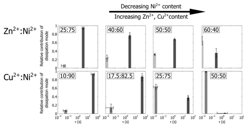
Figure 4. Relative contributions of slow and fast relaxation modes in double metal-ion hydrogels When the total metal concentration is held constant, changing the ratios of \text{Ni}^{2+} ions (slow exchange kinetics) to \text{Zn}^{2+}/\text{Cu}^{2+} ions (fast exchange kinetics) directly modulates the relative contributions of the corresponding slow and fast dissipation modes (dark and light bars, respectively). (top) His- \text{Zn}^{2+}:\text{Ni}^{2+} gels and (bottom) His- \text{Cu}^{2+}:\text{Ni}^{2+} gels. Additionally, it is evident that \text{Cu}^{2+} and \text{Zn}^{2+} have differing abilities to modulate the time-dependent properties of the hydrogels; note especially that \tau_{\text{slow}}(\text{Cu}^{2+}:\text{Ni}^{2+}) \gg \tau_{\text{slow}}(\text{Zn}^{2+}:\text{Ni}^{2+}) and that \tau_{\text{slow}}(\text{Zn}^{2+}:\text{Ni}^{2+}) monotonically decreases with decreasing \text{Ni}^{2+} content. All error bars show the mean \pm standard error, n = 2 except the His-10% \text{Cu}^{2+} :90% \text{Ni}^{2+} points where n = 4 .
