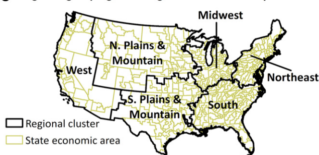
Fig. 1. The geography of intergenerational mobility in the early and late 20th century. Maps of average adult income rank for children born to parents at the 25th percentile in the early 20th century ( A ) and in the late 20th century ( B ) measured at the SEA scale, accompanied by a cluster-based aggregation of outcomes into six regions across both periods ( C ) ( SI Appendix , S15 ). Estimates from the early 20th century are based on the adult income scores for males from the 1900–1915 birth cohorts who were observed in 1920 and 1940 ( A ), and those from the late 20th century are based on estimates for 10 million children from the 1980 to 1982 birth cohorts observed in Internal Revenue Service records in the 1990s and as adults between 2011–2012 ( B ) (see SI Appendix , S12 for discussion of measures). Maps were rendered using the Lambert Conformal Projection.
