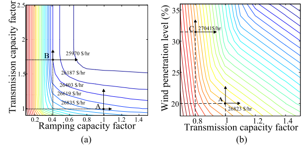
Fig. 7. (a) Relation between ramping and transmission. (b) Relation between transmission and wind penetration level.
