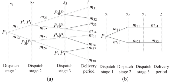
Fig. 3. (a) Scenario tree of the RLUC at DS1. (b) Scenario tree of the traditional two-stage operation at DS1.
