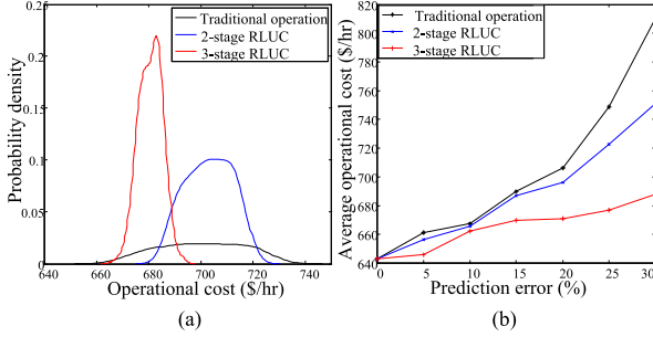
Fig. 5. (a) Comparison on PDFs. (b) Comparison on average operational cost.
