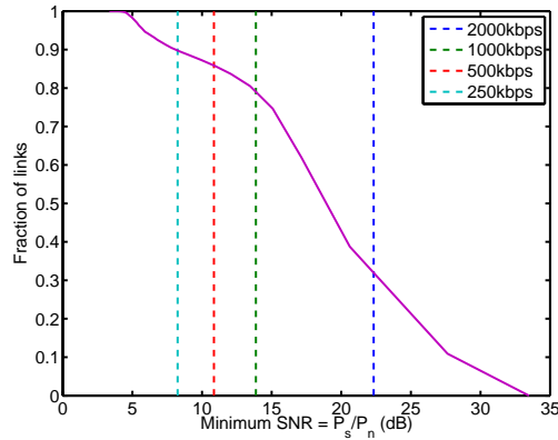
Figure 4.5: The complimentary CDF shows the fraction of links in the network having SNR greater than indicated. The vertical dashed lines show the minimum SNRs required for standards-compliant performance at various data rates.
