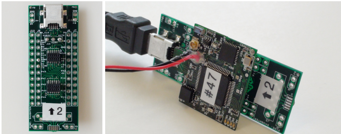
Figure 2.5: A break-out daughter board, with additional expansion headers and a USB interface, allows the GINA mote to be connected to a standard breadboard or scope probes for quick prototyping.
