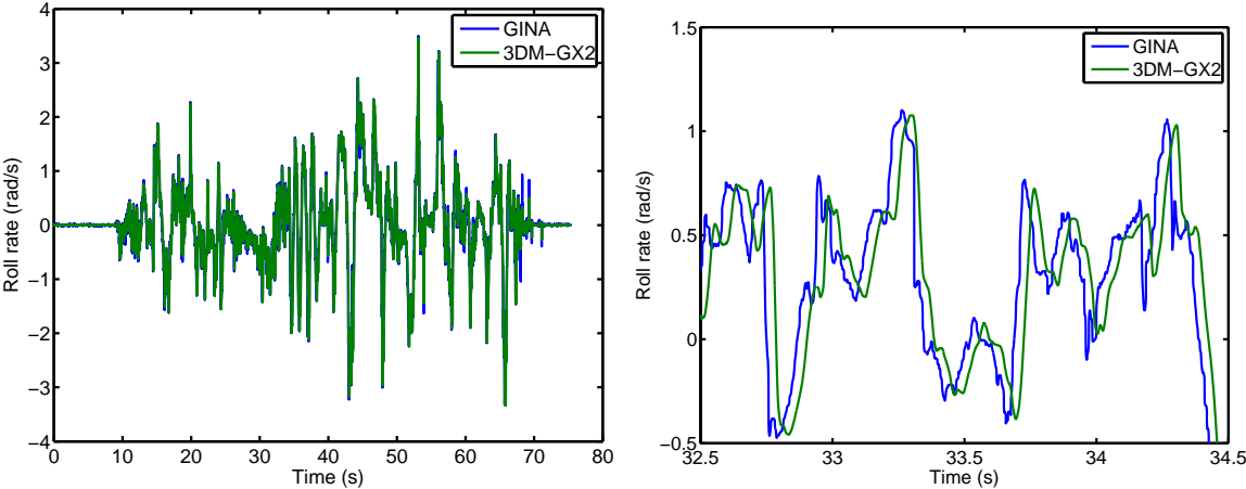
Figure 2.9: A comparison of the GINA and 3DM-GX2 angular rate measurement.
