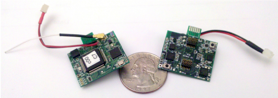
Figure 2.1: GINA provides inertial sensing, processing, control, and wireless communication on a board smaller and lighter than a US quarter.
