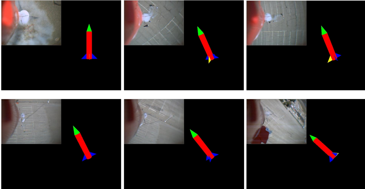
Figure 3.5: Inertial sensor data postprocessed from a rocket launch show the state estimate evolving along with the actual body motion, captured by an on-board camera.
