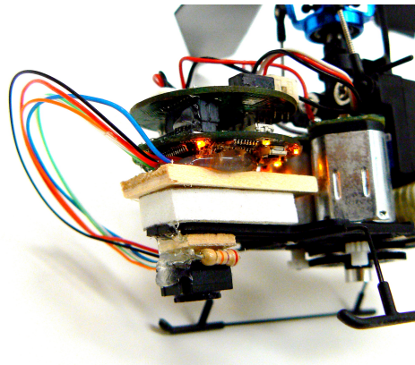
Figure 3.18: A downward pointing WiiMote camera is wired into a serial port on the GINA controller to enable the helicopter to hover over the IR beacon.
