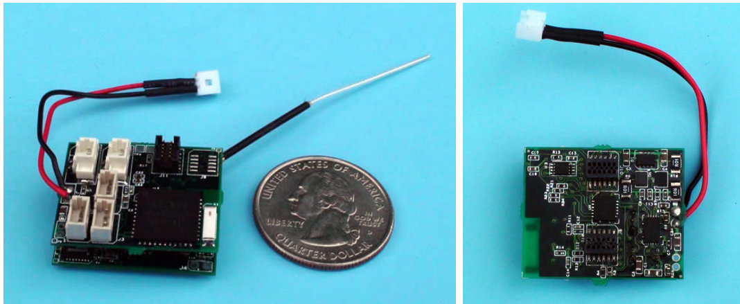
Figure 2.6: A daughter board for the GINA mote brings PWMs out to connectors for servos, uses other PWMs for brushed motor controllers, and includes additional sensors such as a battery fuel gauge, GPS receiver, and vision processors.
