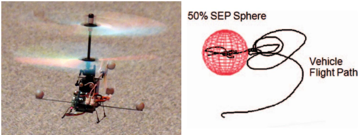
Figure 3.15: The Walkera 5G6 coaxial helicopter is shown using the WARPWING system with VICON position feedback to autonomously hover. The silver balls are the reflectors used by the vision based motion capture system. On the right, a sample flight path from [60] is plotted in space using the VICON data.
