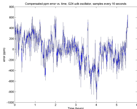
Figure 4.8: The frequency of an on-chip relaxation oscillator drifts mostly between \pm 600 ppm. Image and data courtesy Mark Lemkin, used with permission [29].
