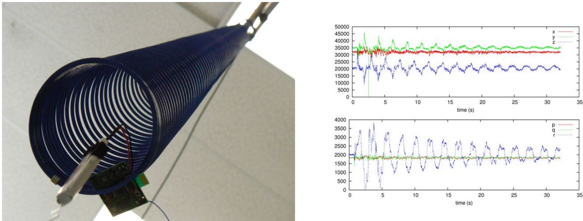
Figure 2.14: Inertial data collected from a GINA mote mounted on a coiled spring, demonstrating both oscillatory rotation and translation. Data courtesy Thomas Watteyne [54].
