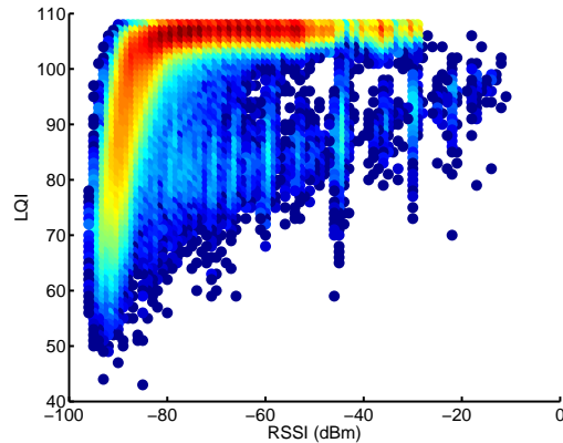
Figure 4.2: The number of links at a given RSSI and LQI is shown in this log-rhythmic density plot. Red points indicate numbers on the order of 10^4 while dark blue points indicate numbers on the order of 10^0 .
