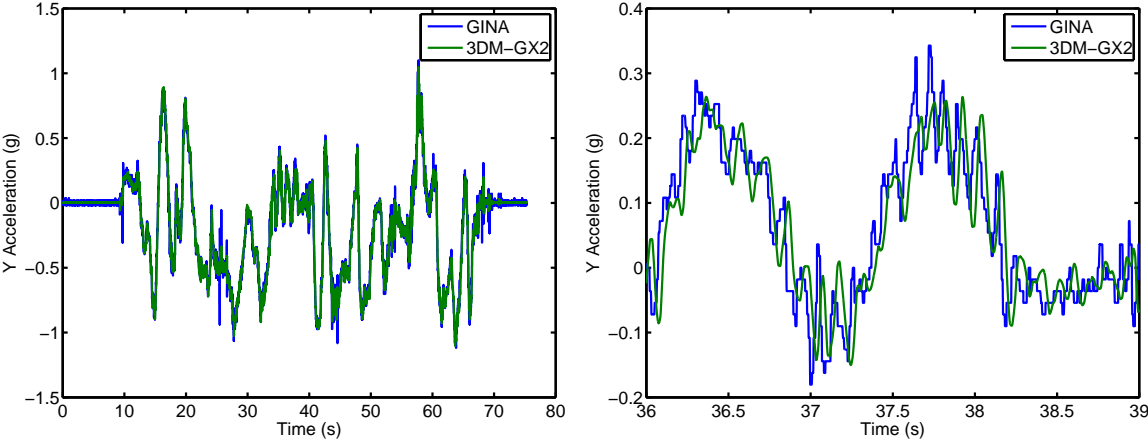
Figure 2.10: A comparison of the GINA and 3DM-GX2 acceleration measurement.
