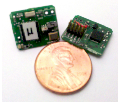
Figure 2.7: GINA 4.0 is the newest development in the hardware series, employing the latest integrated hardware solutions to significantly miniaturize the system.
