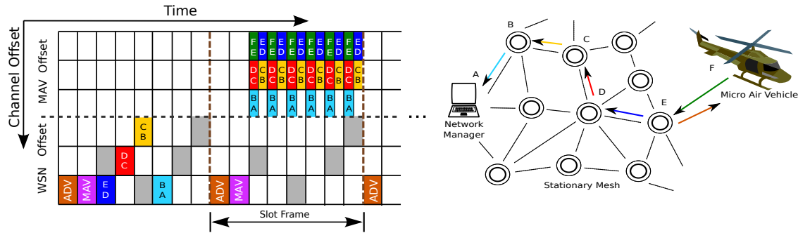
Figure 5.5: In burst mode, the nodes along the direct path from the MAV to the base station remove themselves from the TSCH network and communicate in a separate high throughput, low latency mode.
