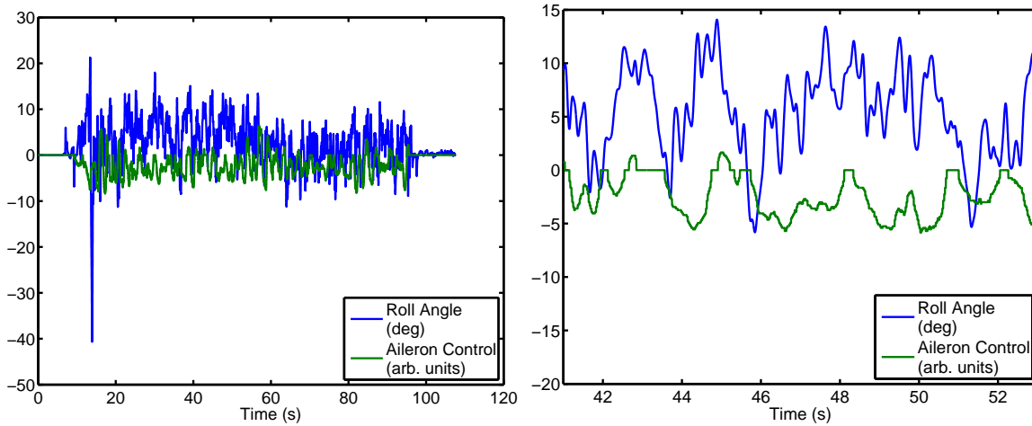
Figure 3.14: A trace of the roll angle during a controlled flight displays a time-varying attitude setpoint over the course of a hover. Comparison to the controller input reveals a dependence on additional states.
