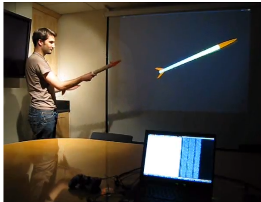
Figure 3.6: GINA sensor data transmitted wirelessly to a laptop base station is integrated in real time to give a 6DOF state estimate. The estimated attitude is projected alongside the physical system demonstrating excellent agreement a posteriori.
