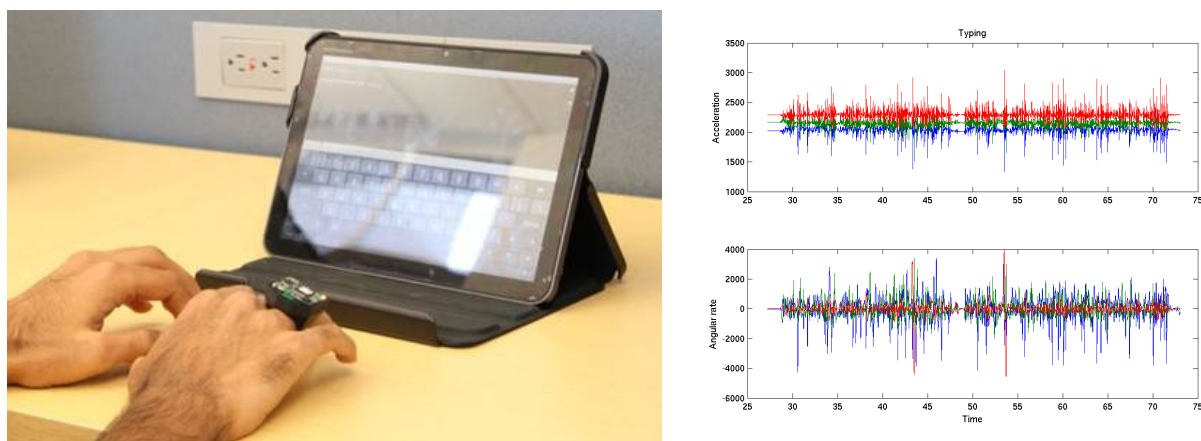
Figure 2.17: The WARPWING code can gather inertial data from the RinGINA, measuring 6DOF state and dynamic motion. Custom software can be written to translate the data into virtual keypresses, potentially replacing a physical keyboard with a body-mounted IMU.
