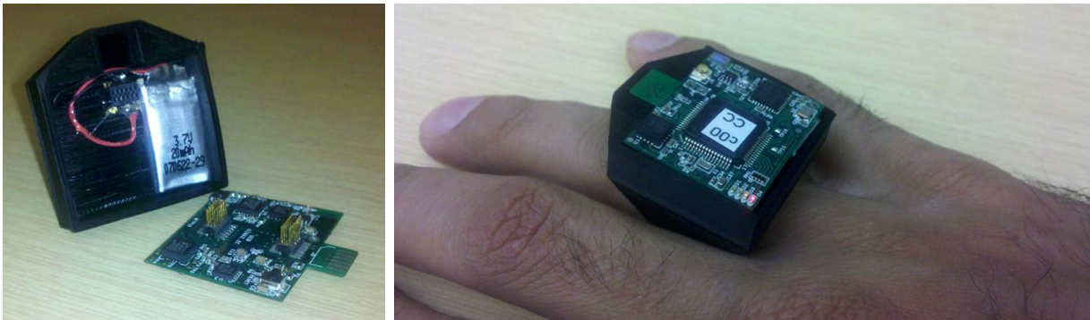
Figure 2.16: The RinGINA device contains a GINA mote on a custom manufactured ring. The WARPWING platform was used to quickly develop an unobtrusive wireless body-mounted sensor.
