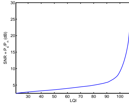
Figure 4.3: Simulation results returning LQI across SNR can be inverted to predict SNR given LQI, as shown in this plot. At high SNR, the integer-level granularity of LQI results in lower SNR resolution.
