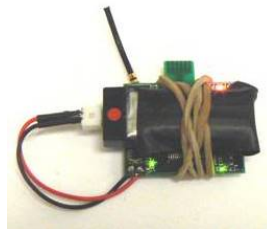
Figure 2.20: This small lightweight footstep detector is designed from the schematic level on up using the WARPWING system as a base, but replacing the accelerometer with one far more sensitive.
