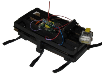
Figure 2.19: DASH, a small, lightweight crawling robot developed at UC Berkeley, uses the WARPWING system to measure inertial rates and motor back EMF for dynamic analysis and control.
