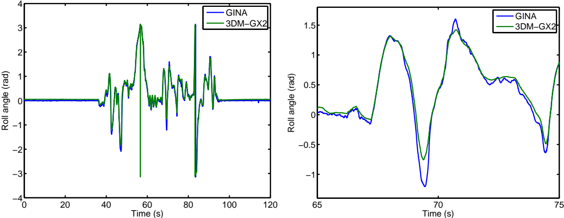
Figure 2.11: Roll angle estimate comparison. GINA and 3DM-GX2 agree closely in their state estimates.
