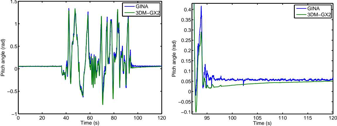
Figure 2.12: Pitch angle estimate comparison. The noisier GINA estimate also allows a much shorter settling time than the 3DM-GX2.
