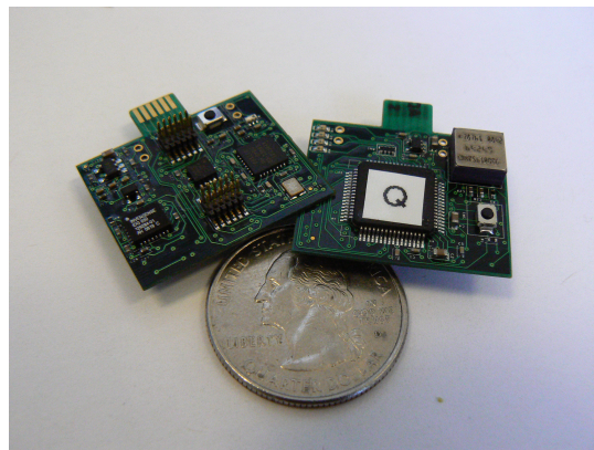
Figure 2.3: GINA 2.0, the first design in the current GINA 2.x series, has undergone several revisions to yield the current version GINA 2.2c shown in figure 2.1
