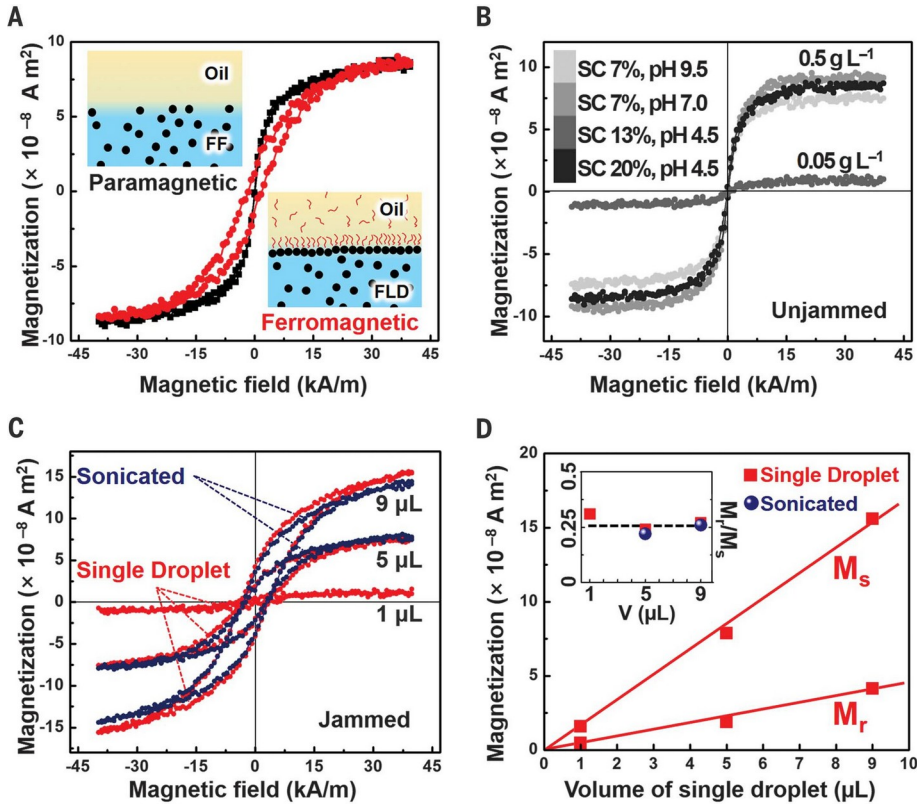
Fig. 1. Tunable transformation of a paramagnetic FF into an FLD by the interfacial jamming of MNP-surfactants. (A) Magnetic hysteresis loops of droplets with (red line) and without (black line) an interfacial layer of jammed MNP-surfactants measured with a vibrating sample magnetometer. Two schematics of aqueous FF and FLD, containing \text{Fe}_3\text{O}_4\text{-CO}_2\text{H} MNPs ( 0.5 \text{ g L}^{-1} ) at pH 4.5, immersed in toluene without and with POSS- \text{NH}_2 ligands ( 1.0 \text{ g L}^{-1} ). (B) Hysteresis loops of individual 5-mL aqueous droplets, with 0.5 \text{ g L}^{-1} and 0.05 \text{ g L}^{-1} of \text{Fe}_3\text{O}_4\text{-CO}_2\text{H} MNPs at different pH, immersed in 0.01 \text{ g L}^{-1} ligand solution. Surface coverage (SC) of droplets is \sim 7 to \sim 20\% where MNPs assemblies are not jammed. (C) Hysteresis loops of single, jammed aqueous droplets with 0.5 \text{ g L}^{-1} of MNPs at pH 4.5 immersed in a 1.0 \text{ g L}^{-1} solution of POSS- \text{NH}_2 in toluene and hysteresis loops of the same system after being sonicated (figs. S1 and S2). (D) M_r and M_s of the droplets as a function of droplet volume. In the inset, the remanence ratio M_r/M_s as a function of initial droplet volume (single droplet or droplet sonicated into multiple smaller droplets) remains constant at \sim 0.25 . FF, ferrofluid; FLD, ferromagnetic liquid droplet.
