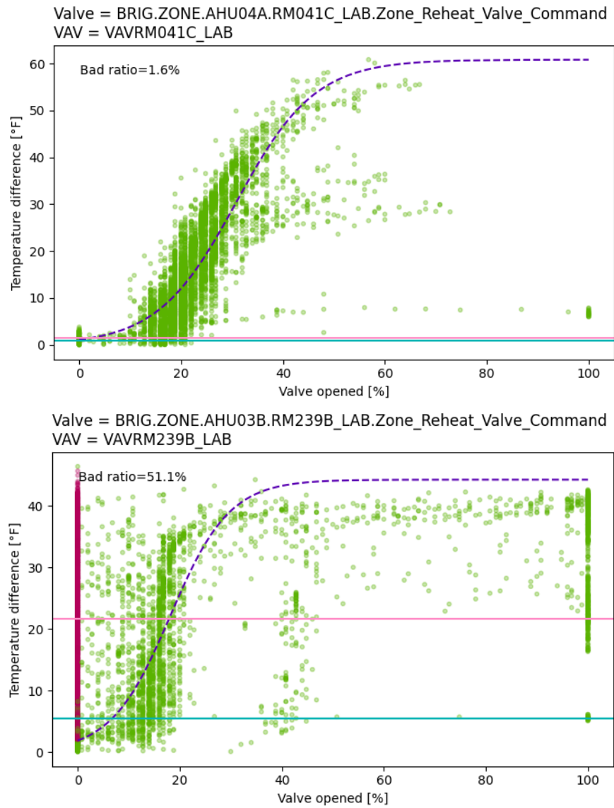
Figure 20: Using Brick to enable the detection of malfunctioning valves
