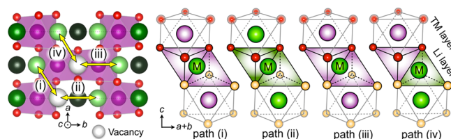
Figure 2. Illustration of the four symmetry-distinguishable migration paths (i), (ii), (iii), and (iv) as indicated by their local cation environment.
