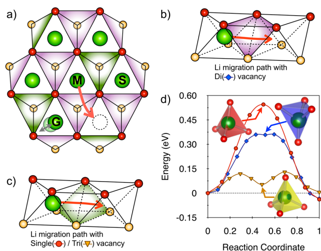
Figure 3. (a) Schematic illustration of the Li-layer with a mobile Li-ion (marked as M) and the gate Li (marked as G). (b) A divacancy mediated Li passing through the T_{4g}^{\text{Li}} site and (c) a single- and trivacancy mediated Li passing through the T_{2b}^{\text{Li}} site. (d) The Li migration energy as a function of neighboring single-, di-, and trivacancy clusters.
