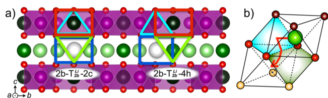
Figure 4. Illustration of the possible migration paths for interlayer (TM to Li layer) Li migration. Cyan indicates the T_{2c}^{\text{TM}} and T_{4h}^{\text{TM}} TM tetrahedral sites and green the Li-layer T_{2b}^{\text{Li}} site.
