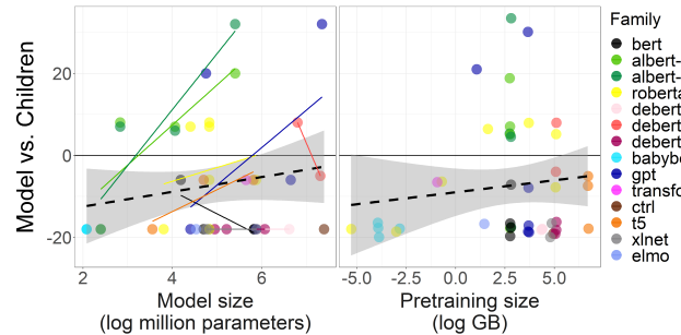
Figure 3: Models' distance from children by model size and pretraining size, in Rabagliati et al. (2013) experiment 2.
