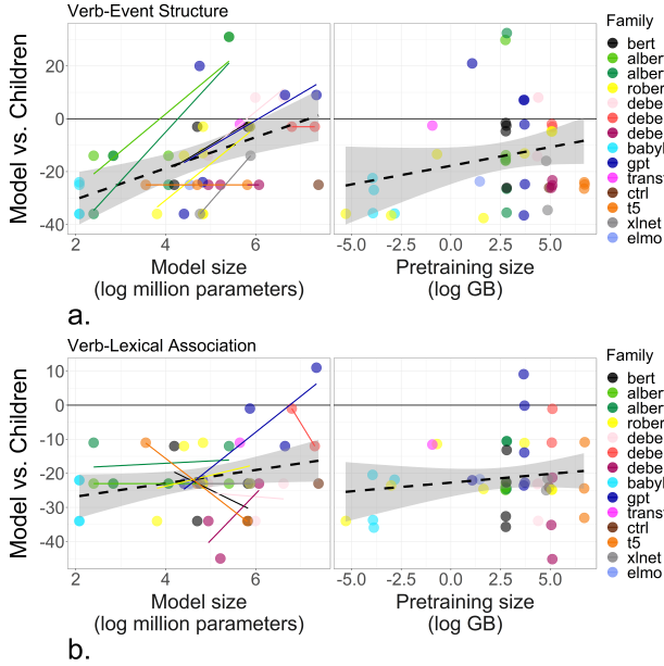
Figure 4: Models’ distance from children by model size and pretraining size, when comparing verb-event vs. control (a) and verb-lexical vs. control conditions (b).
