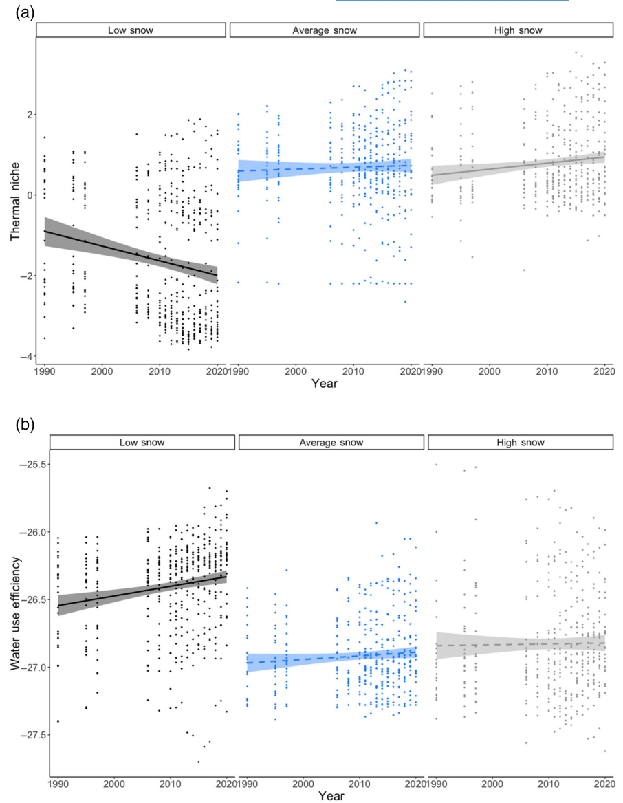
FIGURE 3 Community-weighted (a) mean annual temperature niche (°C) and (b) water-use efficiency values (WUE; \Delta \delta^{13}C ) through time for the three snow depth groups. Points indicate a community-weighted mean for each plot in each time point. Dashed lines indicate nonsignificant trends ( p > 0.05 ) through time; solid lines indicate significant trends through time. 95% confidence intervals based on ordinary least-squares linear regression are shown as shaded areas around the trend lines.
