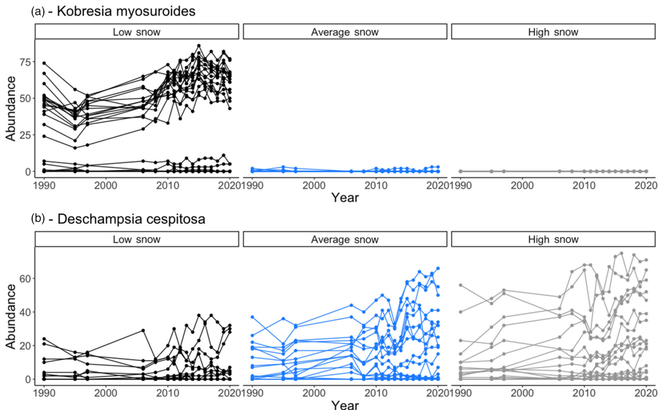
FIGURE 4 Abundance (number of hits) of the two dominant species across the saddle plots (a) Kobresia myosuroides and (b) Deschampsia cespitosa through time within each snow depth group. Points represent plot-level measurements at each time point.
