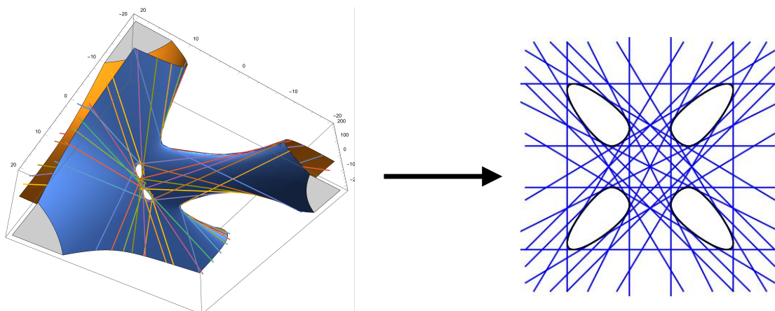
Figure 1: The projection \pi : \text{Bl}_p(S) \rightarrow \mathbb{P}^2 of the blowup at a point p of a smooth cubic surface S is a 2-sheeted branched cover, branched over a smooth plane quartic C . The branching locus in S is the inner rim of each of the four holes in S , two of which go off to infinity in the left-hand picture. The image \pi(C) of each of the 27 lines in S is a bitangent of C . Here we see (the real points of) a branched cover given by projection to the plane of the paper. The left part of the figure is taken from [SS]; the right from [PSV].
