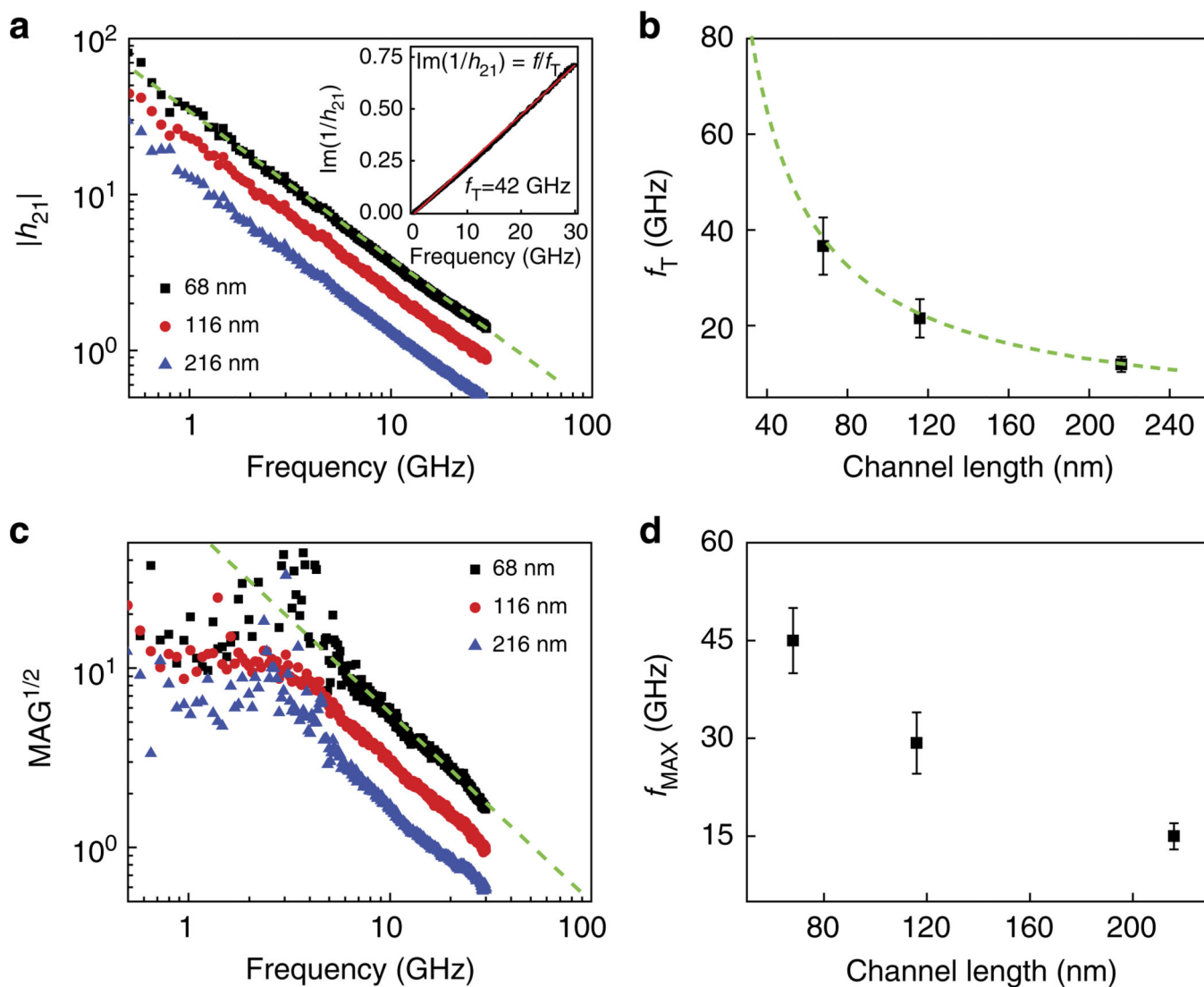
Figure 3. RF performance of the self-aligned MoS 2 transistors
