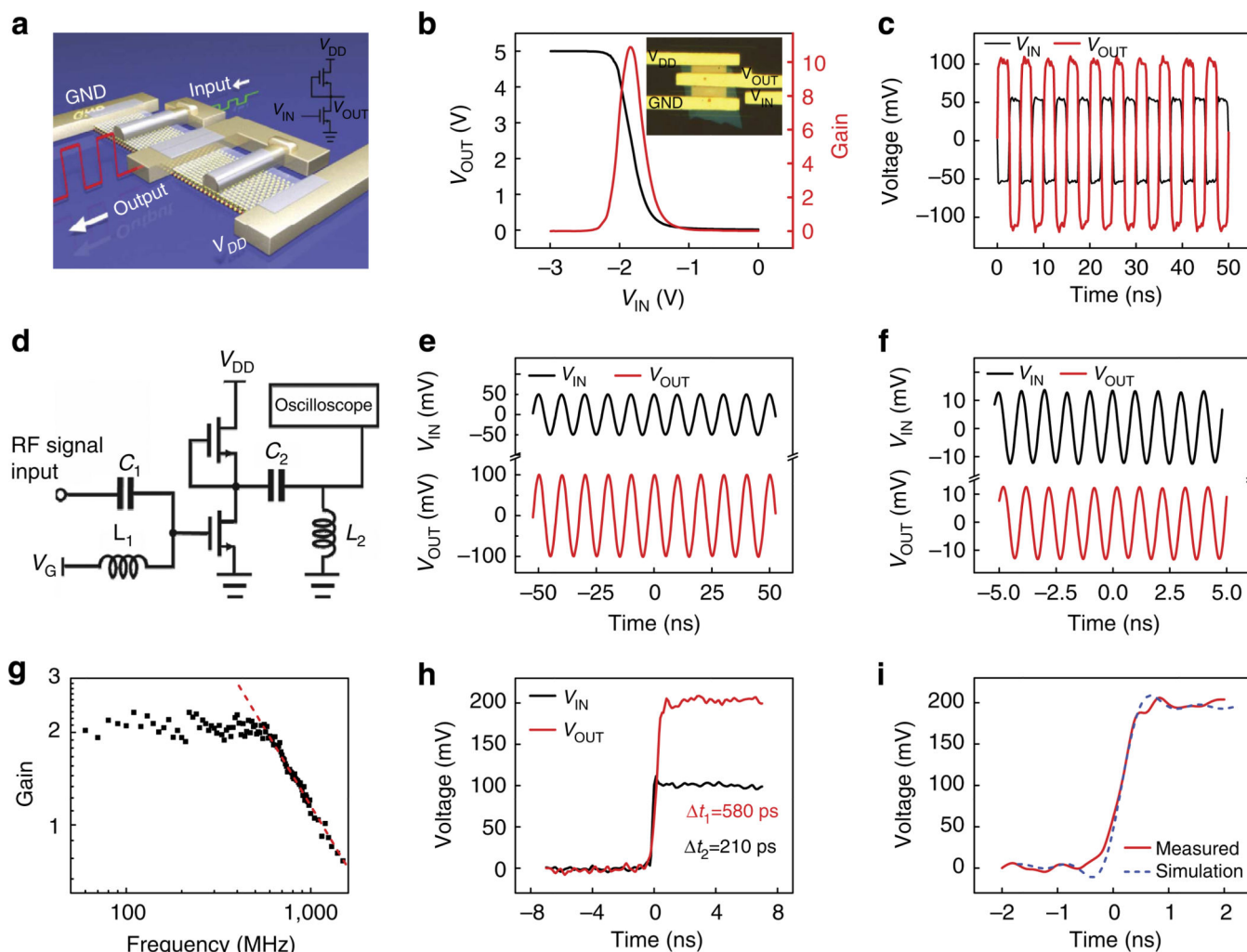
Figure 4. Gigahertz logic inverter and signal amplifier based on MoS 2 transistors on quartz substrate
