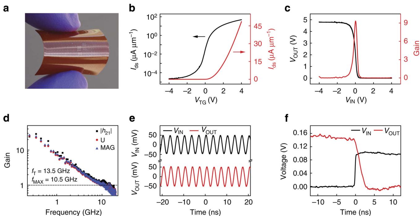
Figure 5. Flexible MoS 2 transistors, integrated logic inverter and RF amplifier
