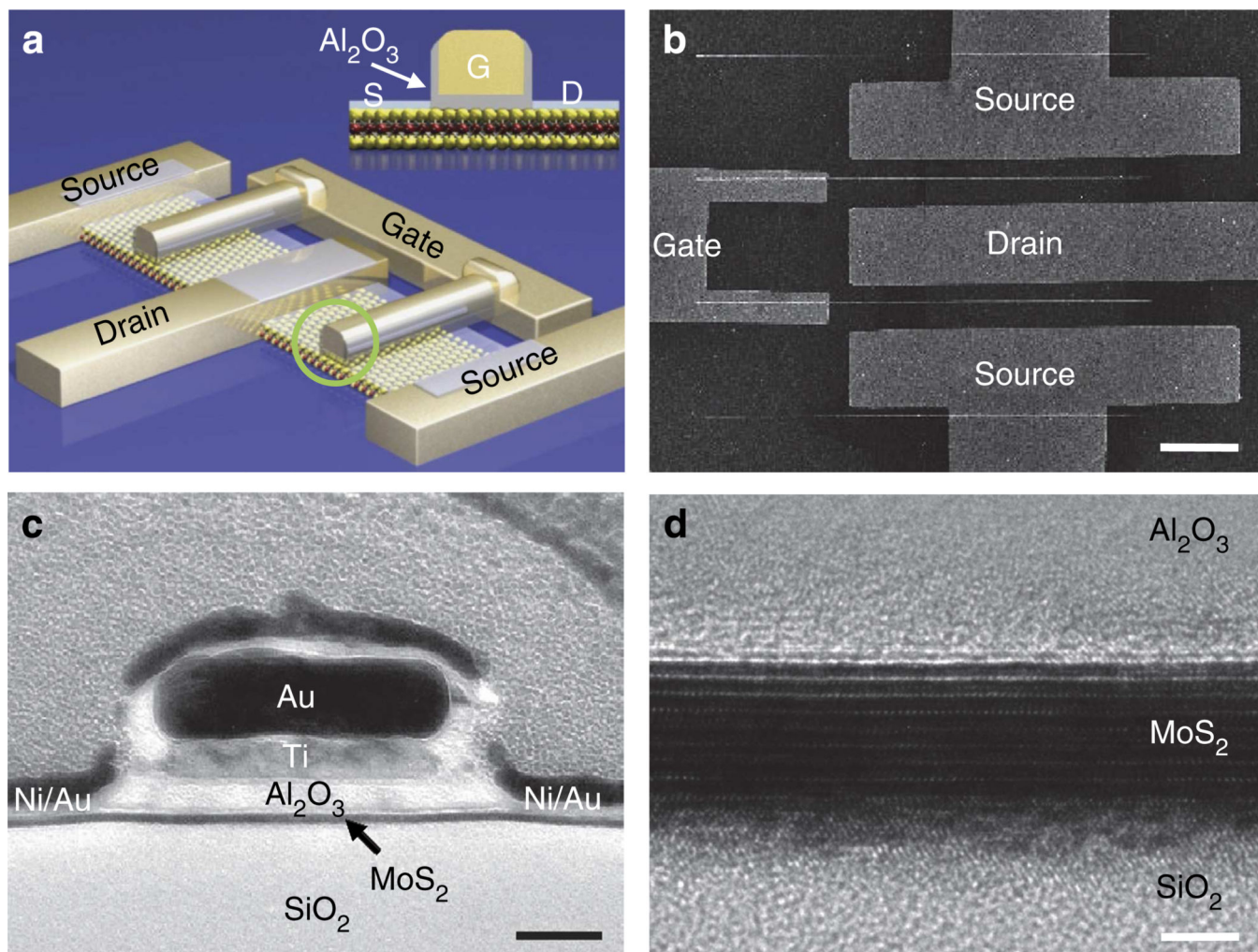
Figure 1. Schematic illustration and characterization of the self-aligned MoS 2 transistors (a) A schematic illustration of a dual-channel self-aligned MoS 2 FETs with transferred gate stacks, and the inset shows the schematic cross-section of the self-aligned device. (b) The SEM image of MoS 2 FETs with transferred gate stacks. Scale bar, 5 μm. (c) The cross-sectional TEM image of a typical self-aligned device. Scale bar, 50 nm. (d) HRTEM image of the interface between MoS 2 and the transferred gate stack. Scale bar, 3 nm.
