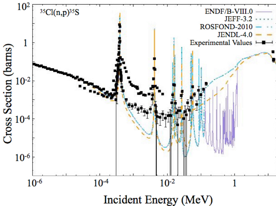
FIG. 1. Comparison of nuclear data libraries for the ^{35}\text{Cl}(n,p)^{35}\text{S} reaction and experimental values [5, 6, 9–11]. Note that ENDF/B-VII.1 is not shown separately as it is identical to ENDF/B-VIII.0.
