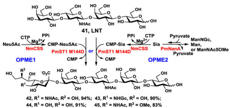
Scheme 5. Synthesis of Sialylated LNT Using OPME Sialylation Systems.
