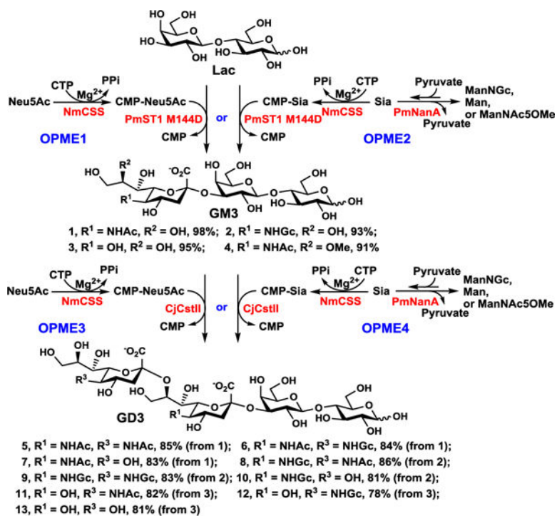
Scheme 2. Production of GM3 and GD3 Glycans Using OPME \alpha 2–3- and \alpha 2–8-Sialylation Systems.
