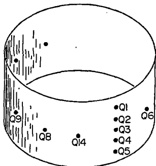
Fig. 1. Location of small coils for initiating and detecting quench propagation.
