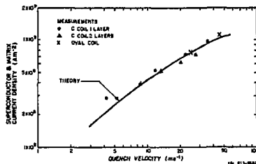
Fig. 2. Predicted and measured quench velocities as a function of the wire current density.
