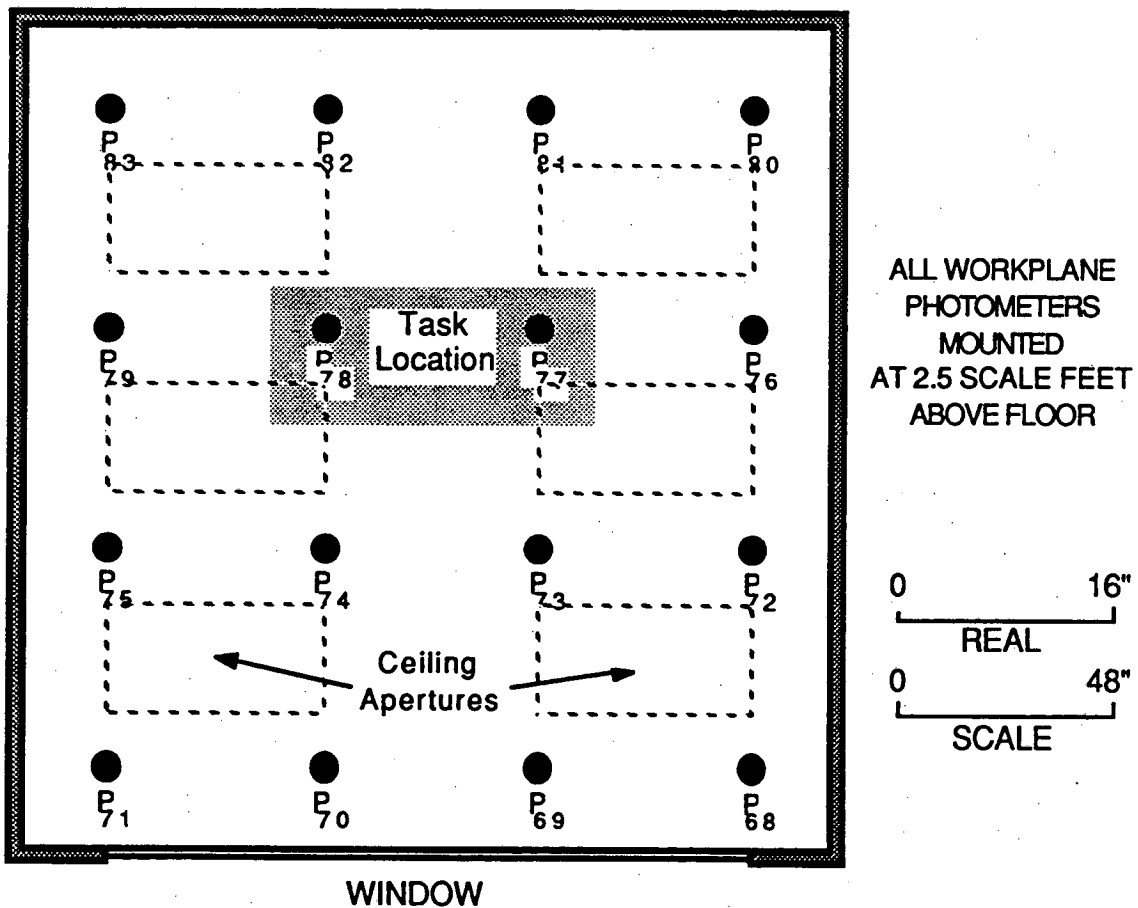
Figure 5. Floor plan and reflected ceiling diagram of small office model. The task illuminance was considered to be the average of the illuminances measured at station points P77 and P78.
