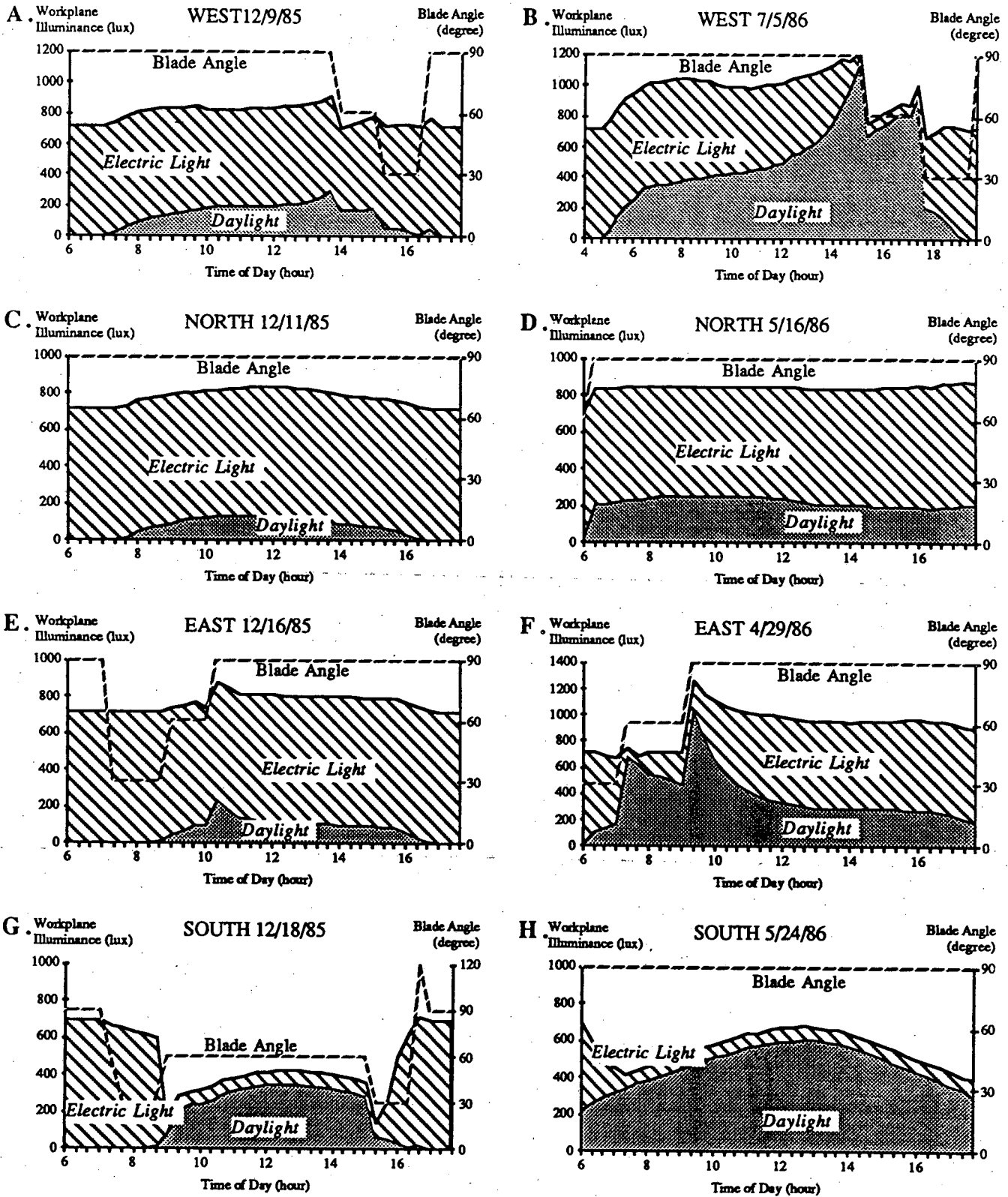
Figure 14. Light levels on workplane for open-loop proportional control systems controlled by window-aimed photosensor for small office model model facing all directions (clear days). Target light level is 720 lux.
