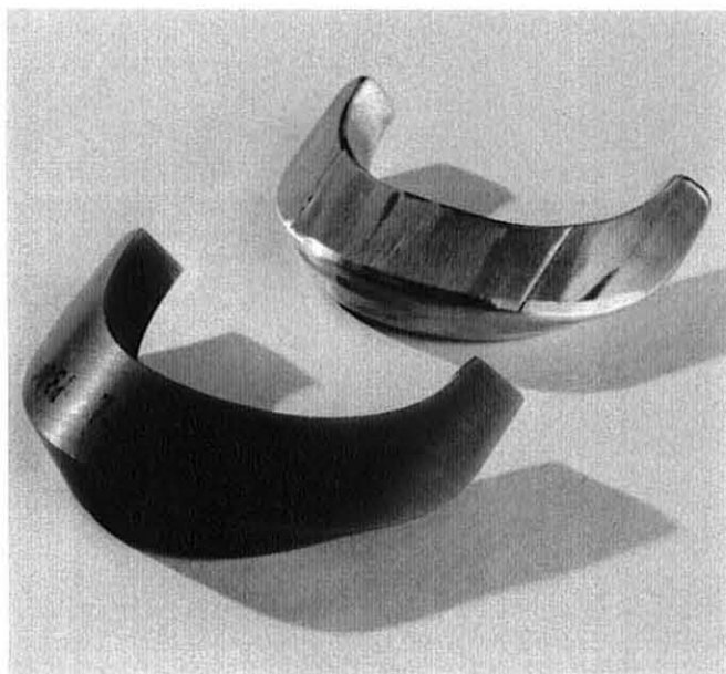
Fig. 5. View of a wax spacer and one casted out of bronze.
