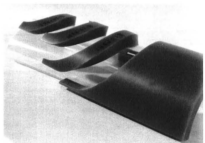
Fig. 4. View of WAX spacers machined by a 5-axis milling machine.
