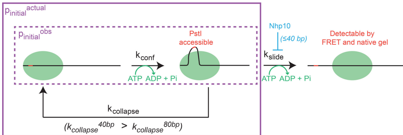
Figure 5. Model for the length-dependent regulation of sliding by INO80 Dashed purple box indicates the steps in the reaction detected by smFRET under continuous laser illumination ( p_{\text{initial}}^{\text{obs}} ). Solid purple box indicates p_{\text{initial}}^{\text{actual}} , which encompasses all of the events that precede translocation in our model, including the length-sensitive k_{\text{collapse}} pathway that is too slow to be detected by smFRET under continuous laser illumination. For simplicity, we have shown the Nhp10 module to only inhibit k_{\text{slide}} (see also Discussion).
