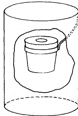
b. BaF_2 CRUCIBLE WITH SUPPORT SYSTEM
