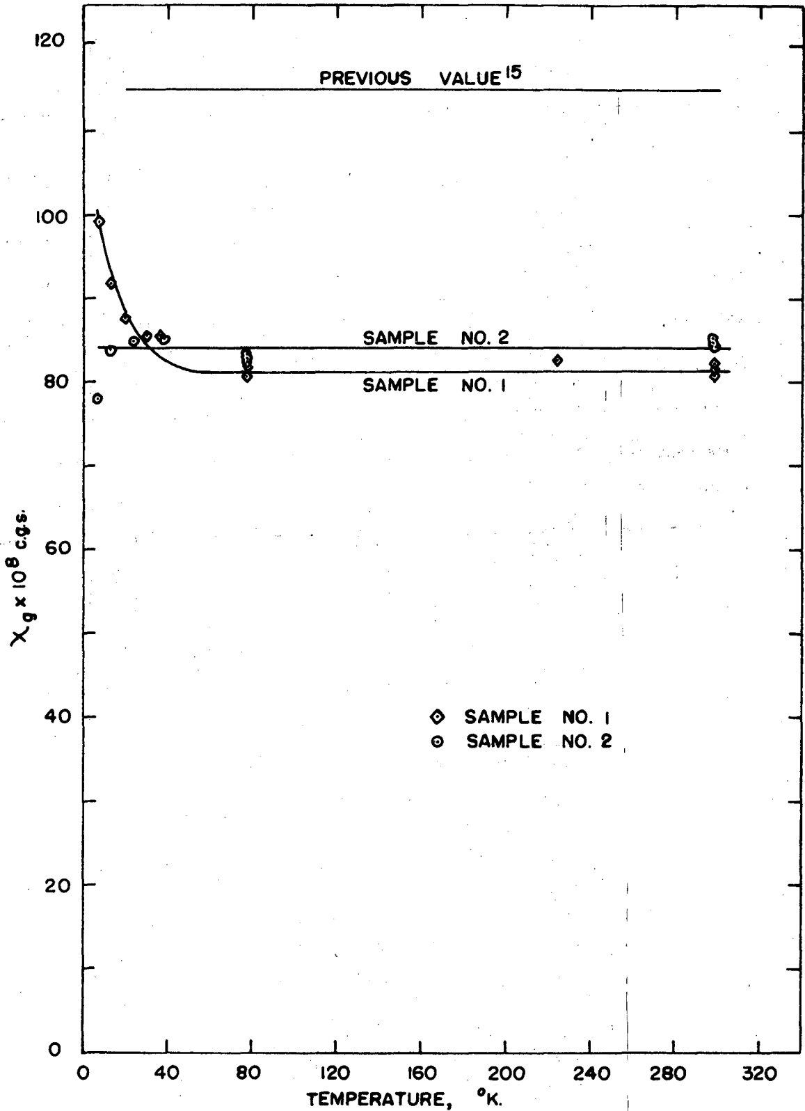
Fig. IX. Magnetic susceptibility of protactinium metal.
