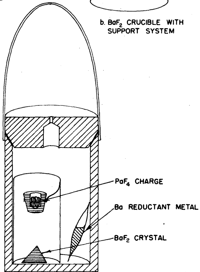
c. LOADED REDUCTION CRUCIBLE SYSTEM
