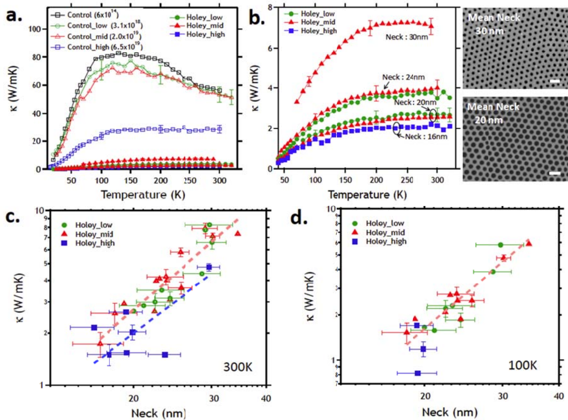
Figure 4. The thermal conductivities of the control silicon ribbons and HS ribbons with different doping levels (boron-doped): 3.1 \times 10^{18} cm -3 (green circles), 2.0 \times 10^{19} cm -3 (red triangles), and 6.5 \times 10^{19} cm -3 (blue squares). Open circles, triangles, and squares are for control silicon ribbons. Solid circles, triangles, and squares are for HS ribbons. (a) The temperature-dependent thermal conductivities of control silicon and HS ribbons with varied doping concentrations. (b) The temperature-dependent thermal conductivities of HS ribbons, which is the enlarged illustration of (a). The mean neck sizes were estimated based on SEM images as shown. Scale bars are 100 nm. (c) The HS thermal conductivities, at 300 K, as a function of the neck size for different doping levels are plotted in log-log scale. The power law fittings are as guide lines for the thermal conductivity of low- and mid-doped HS ribbons combined (dashed red line), and for high-doped HS devices
