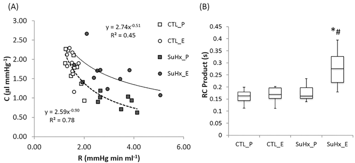
Figure 5. Estrogen modifies the relationship between resistance (R) and compliance (C) in pulmonary vasculature. (A) R-C curves and (B) RC time constant. *, P < 0.05 vs. Control; #, P < 0.05 vs. Placebo.
