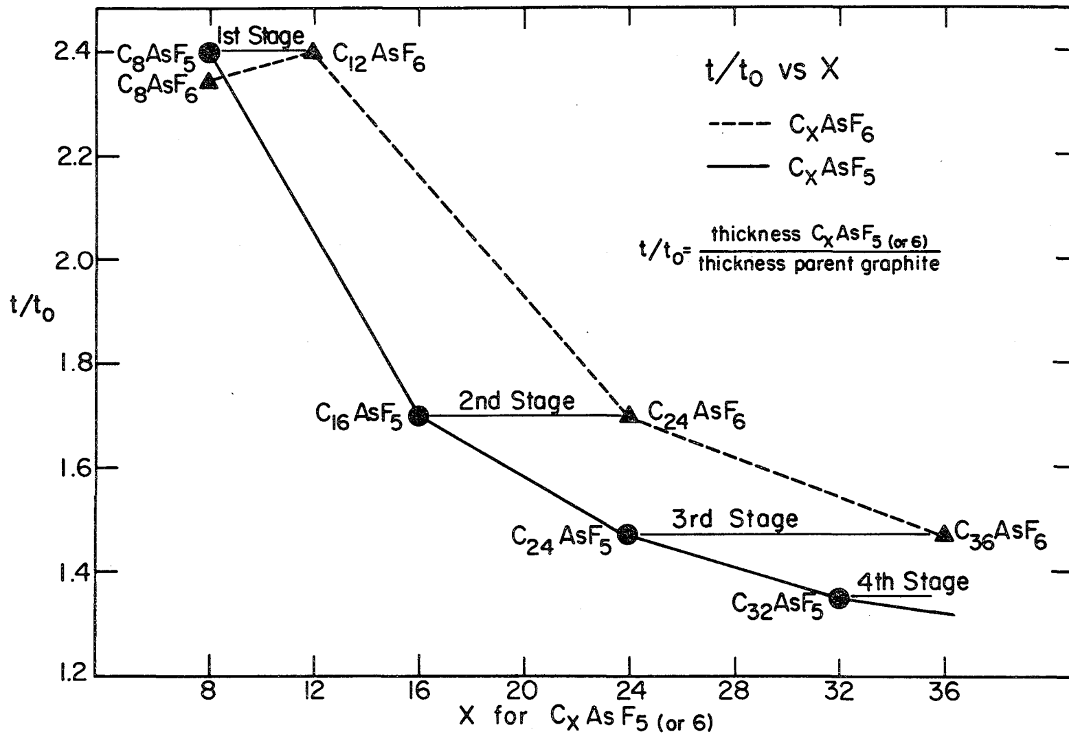
Figure VI-3. Composition/staging relationships for C x AsF 5 and C x AsF 6 .
