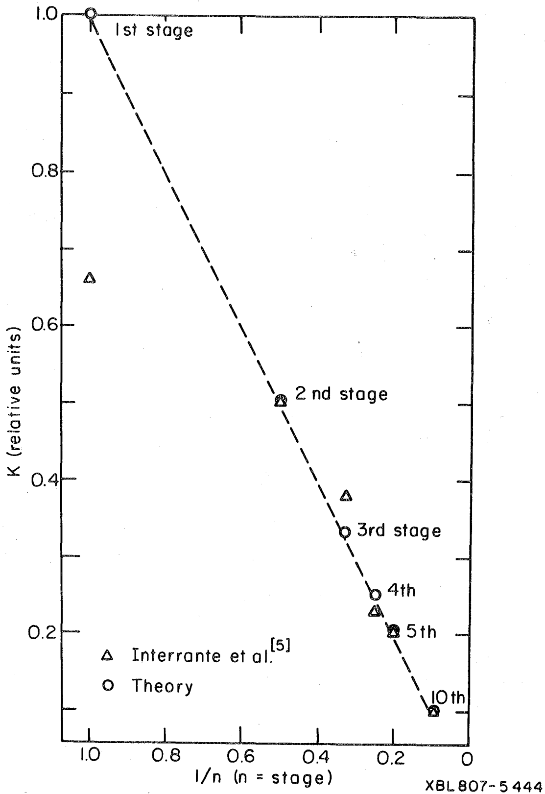
Figure VIII-2. Plots of the conductivity per graphite plane, k , versus 1/n ( n = \text{stage} ) for C_{8n}AsF_5 .
