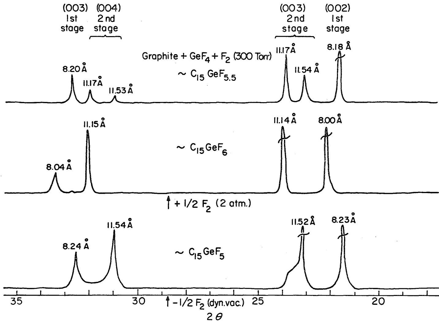
807-5442 Figure VII-1. X-ray diffraction tracings of C 15 GeF 5-6 as a function of fluorine content.
