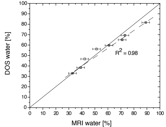
Figure 5: DOS water vs. MRI water.
