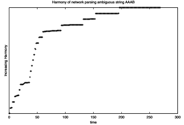
Figure 3: Operation of parsing network on example grammar
