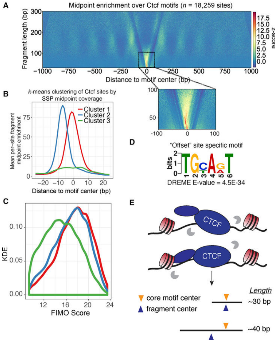
Figure 6. MNase-SSP Enables Dissection of Unique Ctf Binding Modes (A) V plot centered at ENCODE-defined Ctcf motifs. V plots show clearly phased nucleosomes and strong enrichment for short fragment midpoints immediately over the core Ctcf binding motif. Inset: closer inspection of the Ctcf V plot reveals bipartite patterning of fragment midpoints with respect to the core Ctcf motif. (B) k -means clustering ( k = 3) of smoothed (5 bp running mean) per-site fragment midpoint enrichment in a 160 bp window separates >18,000 Ctcf binding sites into distinct clusters. (C) Cluster 3 is separated from clusters 1 and 2 by FIMO score, suggesting that cluster 3 is capturing low-affinity Ctcf binding sites. Distribution differences between clusters 1 and 3 and clusters 2 and 3 are both significant (Kolmogorov-Smirnov: cluster 3 versus cluster 1, D = 0.298; cluster 3 versus cluster 2, D = 0.230; p < 2.2E−16 for both tests). (D) De novo motif detection using the MEME suite uncovers a cluster 2-specific motif, which corresponds to the known motif employed by Ctcf while using zinc fingers 9–11.
