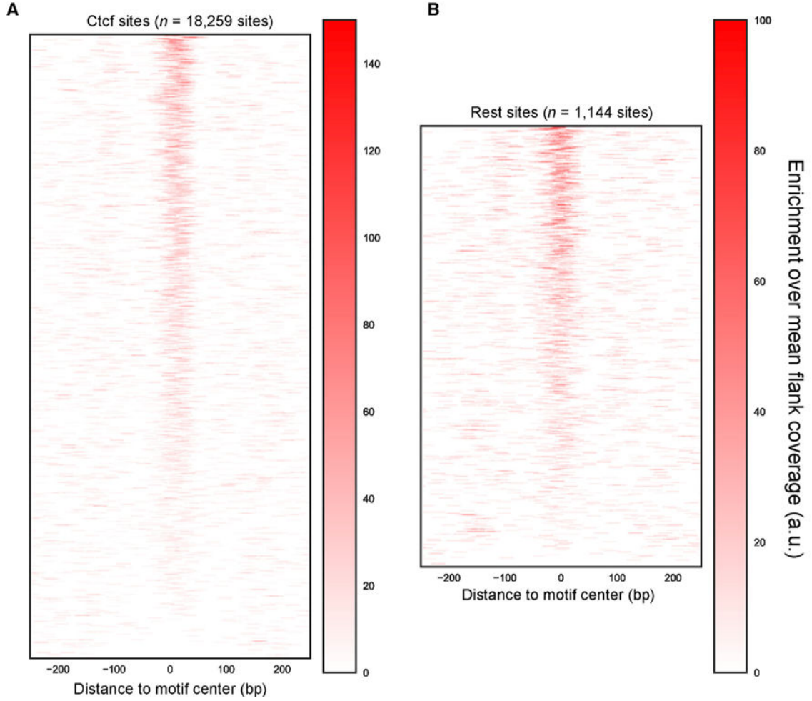
Figure 5. MNase-SSP Short Fragments Footprint Ctf and Rest Binding Sites (A) Heatmap of per-site fragment midpoint enrichment centered at predicted Ctf binding sites for SSP fragments sized between 30 and 59 bp in length. Fragment midpoint enrichment was calculated with respect to a 2 kilobase background coverage distribution, smoothed using a 10 bp running mean, and then plotted in heatmap form sorted by decreasing fragment midpoint enrichment. (B) Heatmap as in (A) but for the transcription factor Nrsf/Rest.
