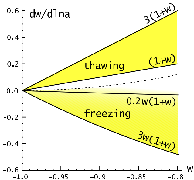
FIG. 1: The w-w' phase space occupied by thawing and freezing fields is indicated by the shaded regions. No strong constraints on this range of dark energy properties exist at present. The fading at the top of the freezing region indicates the approximate nature of this boundary. Freezing models start above this line, but pass below it by a red shift z \sim 1 . The short-dashed line shows the boundary between field evolution accelerating and decelerating down the potential. Future cosmological observations will aim to discriminate between these two fundamental scenarios.
