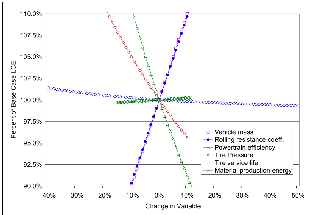
FIGURE 21. Variations in Key Variables Contributing to Tire Life Cycle Energy (LCE), with a Focus on Service Life, Rolling Resistance, Material Production Energy, and Tire Pressure
