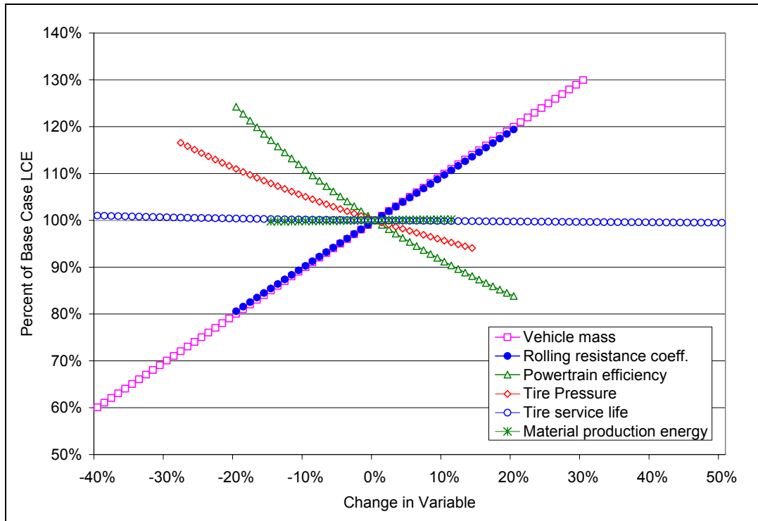
FIGURE 20. Variations in Key Variables Contributing to Tire Life Cycle Energy (LCE)
