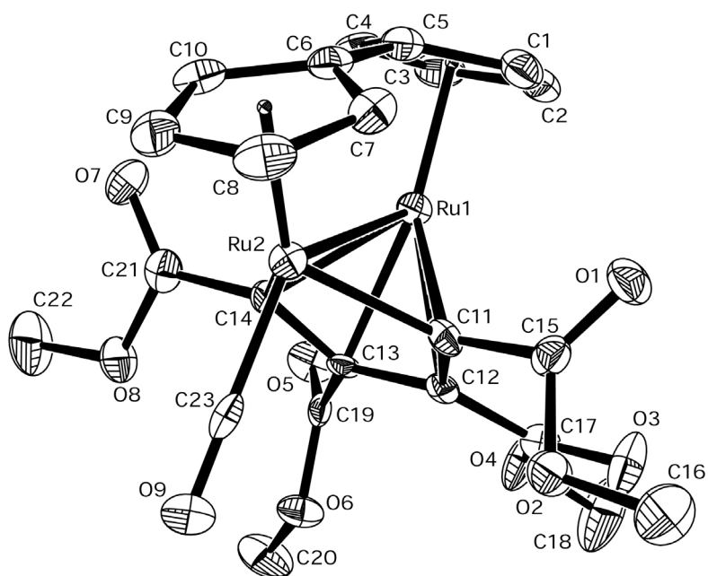
Figure 5. ORTEP diagram of 6 (50% probability surface).
