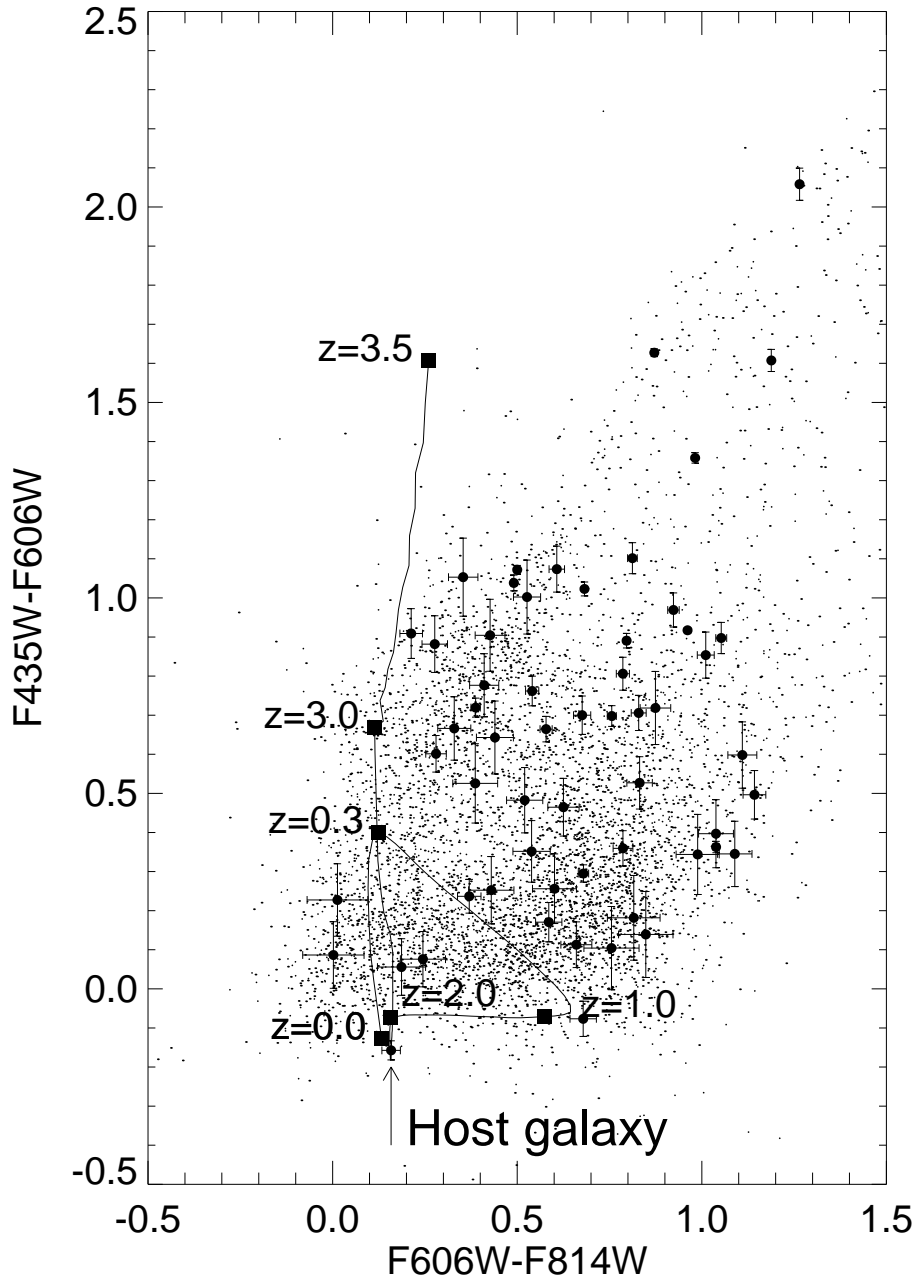
Fig. 6.— The color of the host compared to the colors of galaxies in its environment (filled circles with error bars) and to galaxies in the GOODS South field (dots). Also shown are the colors of the spectral synthesis model shown in Fig. 5 as a function of redshift from z = 0 to z = 3.5 renormalized to go through the host galaxy point.
