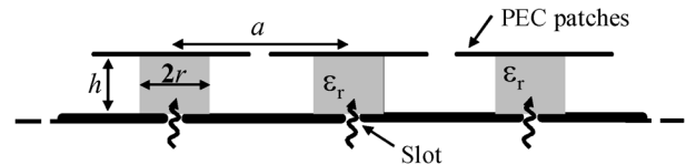
Fig. 1. Lateral view of the array of antennas consisting of metallic patches on the EBG substrate made of a square lattice of dielectric rods in air over a ground plane. The structure acts both as a radiating array and an EBG substrate. Each element is fed by a slot on the ground plane.
