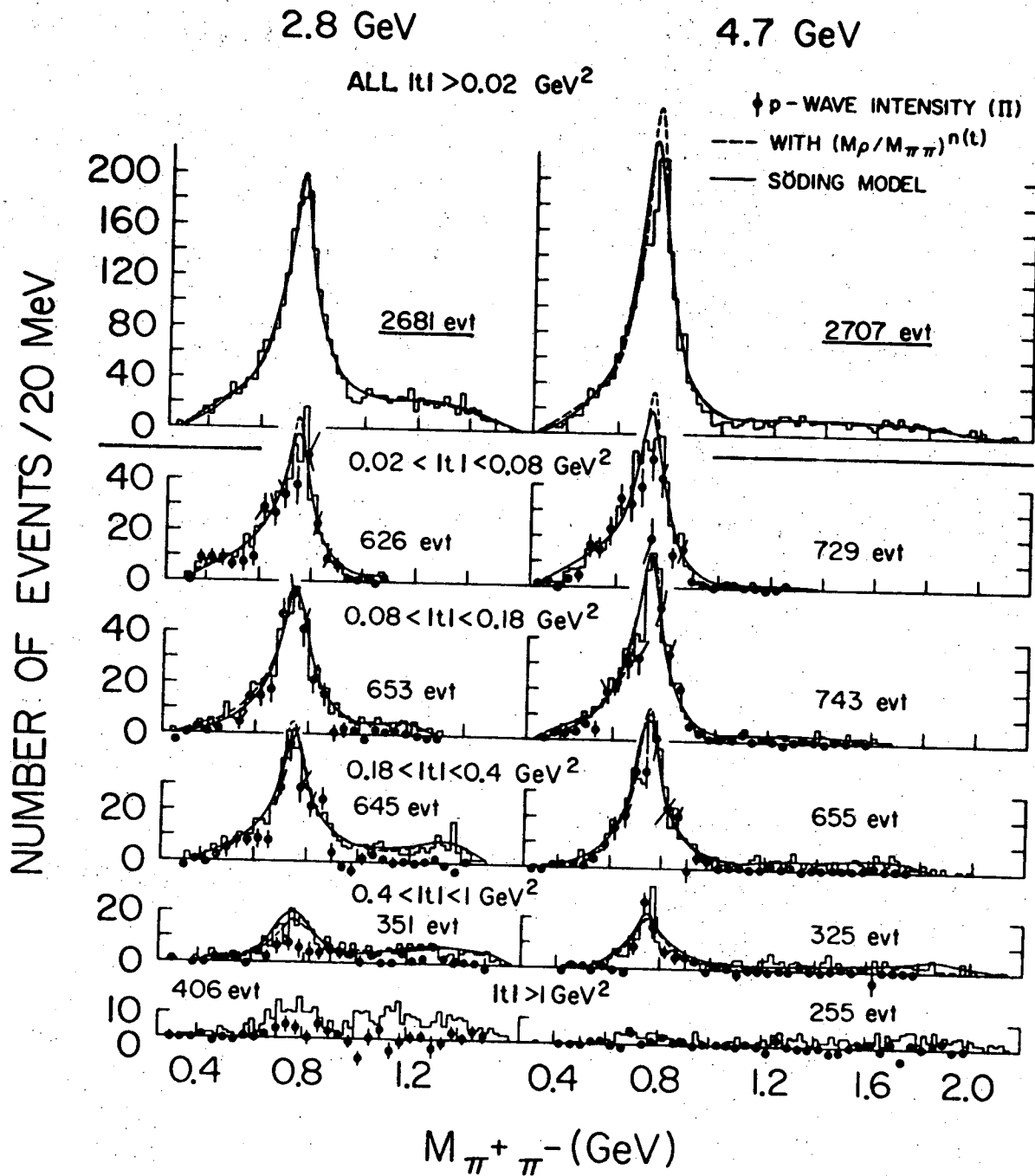
Fig. 9. Reaction \gamma p \rightarrow \pi^+ \pi^- p : \pi^+ \pi^- mass distributions. The helicity conserving p-wave intensity \Pi (see text Eq. 5) is shown by the points ♦. The curves give the results of a maximum likelihood fit using for the \rho^0 the parameterization (M_\rho/M_{\pi\pi})^{n(t)} (----) and the Söding model (—).
