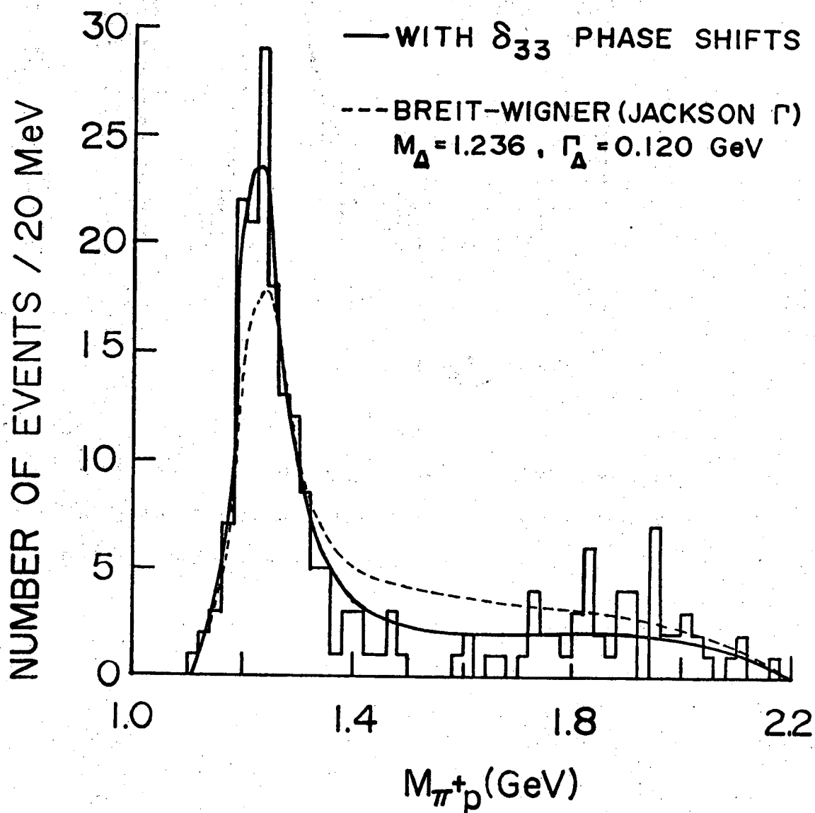
Fig. 30. (b) Reaction \gamma p \rightarrow \pi^+ \pi^- p : M_{\pi^+p} at 2.8 GeV for events with |t_\Delta| < 0.4 \text{ GeV}^2 and M_{\pi^+\pi^-} > 1.0 \text{ GeV} (shaded area of Fig. 30(a) top-left with expanded scale). The curves give the comparison of the \Delta shape with the \delta_{33} phase shifts and a Breit-Wigner shape (Eq. 2.2).
