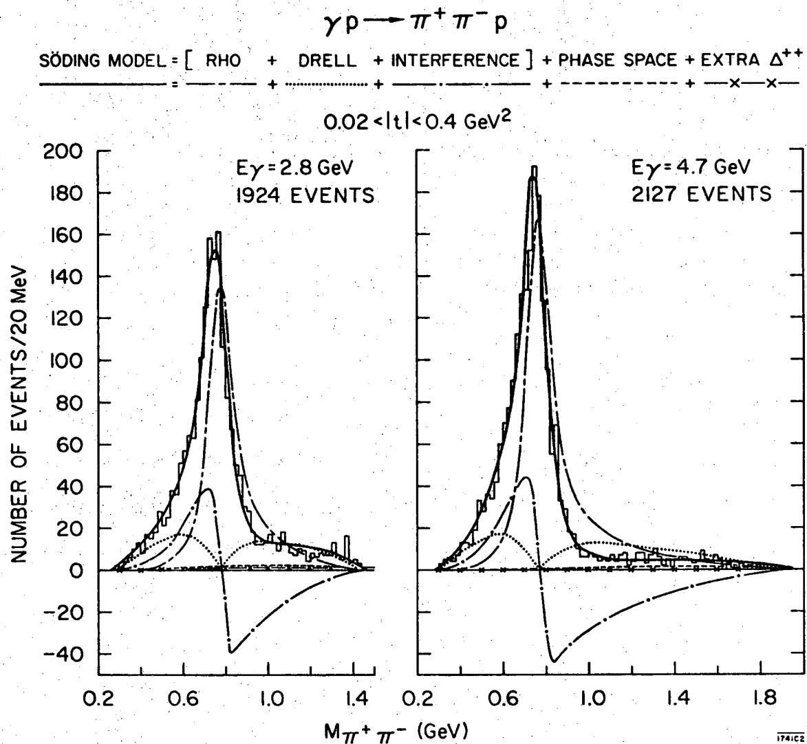
Fig. 16. The \pi^+ \pi^- mass distributions for the reaction \gamma p \rightarrow \pi^+ \pi^- p (data of Fig. 9). The full curve gives the predictions of the Söding Model; the other curves represent the individual contributions making up the Söding Model.
