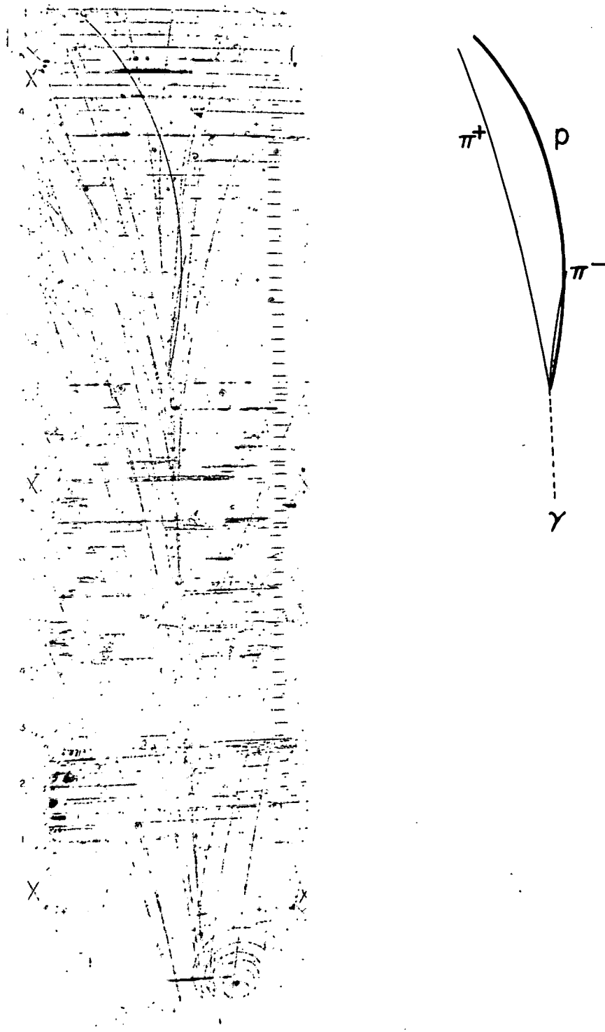
Fig. 2. Typical bubble chamber picture with an event of the reaction \gamma p \rightarrow \pi^+ \pi^- p . The background tracks are electron-positron pairs.
