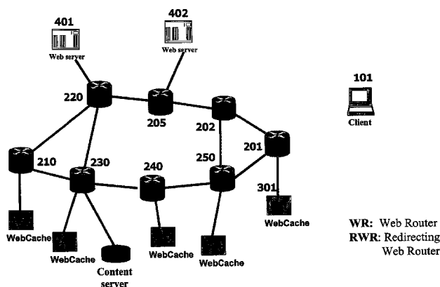
Virtual topology of Web routers
