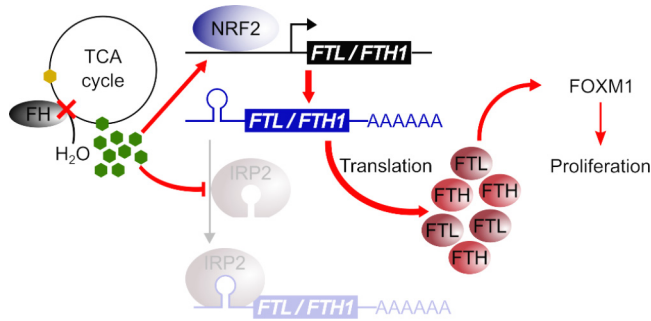
FIG 7 FH inactivation confers chronic proliferative signaling. The diagram shows how FH inactivation increases ferritin levels to promote proliferation. FH , a TCA cycle enzyme that catalyzes the hydration of fumarate (represented by green hexagons) to form malate (represented by yellow hexagons), is inactivated (represented by a red cross) in HLRCC. FH inactivation causes fumarate accumulation. The accumulated fumarate activates the NRF2 transcription factor, which transcribes the ferritin genes FTL and FTH1 . Concurrently, the accumulated fumarate also inhibits IRP2, which normally represses the translation of FTL and FTH1 , leading to a net increase in the ferritin level and subsequent FOXM1-dependent proliferative signaling.
