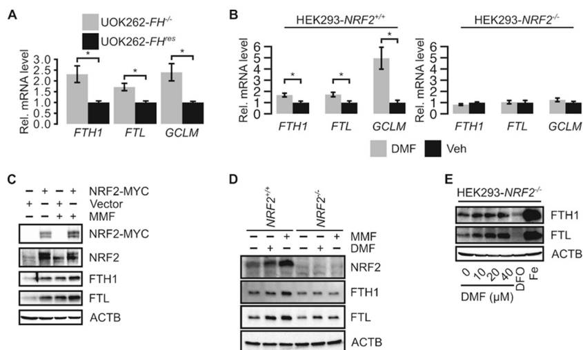
FIG 5 NRF2 activation by fumarate contributes to ferritin accumulation. (A) Quantitative reverse transcription-PCR shows that FH reconstitution in UOK262 (UOK262- FH res ) cells decreases relative FTL and FTH1 transcript levels. Changes in expression levels were normalized to values for UOK262- FH res cells. GCLM is an NRF2 target gene known to be upregulated in HLRC. Error bars represent standard deviations. * indicates a P value of <0.05 as determined by Student's t test. (B) Quantitative reverse transcription-PCR of HEK293- NRF2 -/- and HEK293- NRF2 +/+ cells treated with 40 \mu M DMF or the vehicle (Veh). Changes in expression levels were normalized to values for vehicle treatment. Error bars represent standard deviations. * indicates a P value of <0.05 as determined by Student's t test. (C) Western blot of HEK293 cells transfected with pIRESpuro3 (vector) or NRF2-Myc and treated with the vehicle or 80 \mu M MMF. ACTB was used as a loading control. (D) Western blot of HEK293- NRF2 -/- and HEK293- NRF2 +/+ cells treated with the vehicle, 80 \mu M MMF, or 40 \mu M DMF. ACTB was used as a loading control. (E) Western blot of HEK293- NRF2 -/- cells treated with increasing concentrations of DMF, 200 \mu M DFO, or 200 \mu M Fe.
