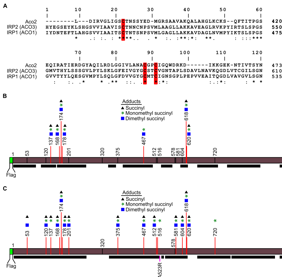
FIG 3 IRP2 is a succination target. (A) Multiple-sequence alignment of mouse Aco2, human IRP2 (ACO3), and IRP1 (ACO1). Succination sites reported for Fh -/- mouse Aco2 are conserved in human IRP1 and IRP2. These sites are highlighted in red. (B) Adduct sites on Flag-tagged wild-type IRP2, as determined by LC-MS/MS. Black bars represent peptides detected by mass spectrometry analysis. (C) Adduct sites on Flag-tagged IRP2-A523R, as determined by LC-MS/MS. Black bars represent peptides detected by mass spectrometry analysis.
