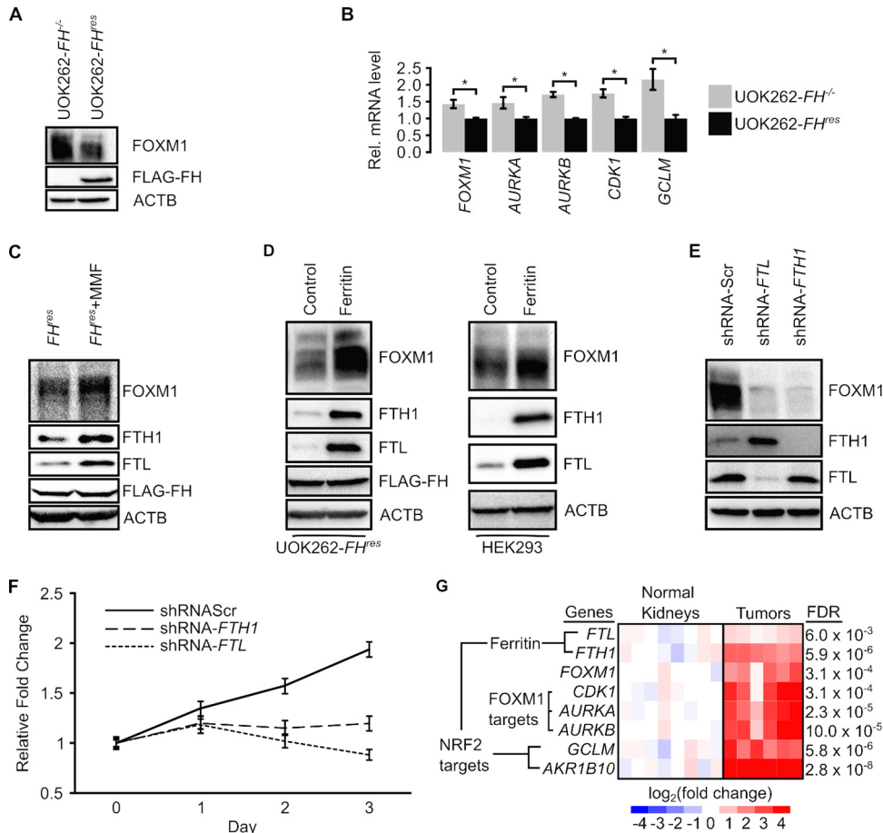
FIG 6 FH inactivation promotes FOXM1 signaling. (A) Western blotting of the FH -inactive UOK262- FH -/- cell line and the FH -reconstituted UOK262- FH res cell line. (B) Quantitative reverse transcription-PCR shows that FH reconstitution in UOK262 cells decreases the relative transcript levels of FOXM1 and its downstream targets AURKA , AURKB , and CDK1 . Changes in expression levels were normalized to values for UOK262- FH res cells. GCLM is an NRF2 target gene known to be upregulated in HLRCC. Data are presented as means ± standard deviations of results from a representative experiment. * indicates a P value of <0.05 as determined by Student's t test. (C) Western blots of UOK262- FH res cells treated with the vehicle or 80 μM monomethyl fumarate show increased FOXM1 signaling with MMF. (D) Western blots of UOK262- FH res cells and HEK293 cells transduced with the pLKO-CMV empty vector (control) or pLKO-CMV- FTL and pLKO-CMV- FTH1 (ferritin) show that ferritin overexpression increases FOXM1 protein levels. (E) Western blots of UOK262 cells transduced with shRNAs targeting FTL (shRNA- FTL ) or FTH1 (shRNA- FTH1 ) show decreased FOXM1 signaling relative to shRNA-Scr, a nontargeting shRNA control. (F) Cell viability measured by formazan production in UOK262 cells after transduction with shRNA-Scr, shRNA- FTL , and shRNA- FTH1 . Data are presented as means ± standard deviations of results from a representative experiment. shRNA- FTL and shRNA- FTH1 knockdown curves were statistically significantly different from the shRNA-Scr curve for shRNA treatment ( P < 0.001) but not for time ( P > 0.05), as determined by two-way analysis of variance. (G) Relative mRNA levels of ferritin genes ( FTL and FTH1 ), FOXM1, FOXM1 target genes ( CDK1 , AURKA , and AURKB ), and nonferritin NRF2 targets ( GCLM and AKR1B10 ) in HLRCC tumors and in normal kidney tissues. FDR, false discovery rate.
