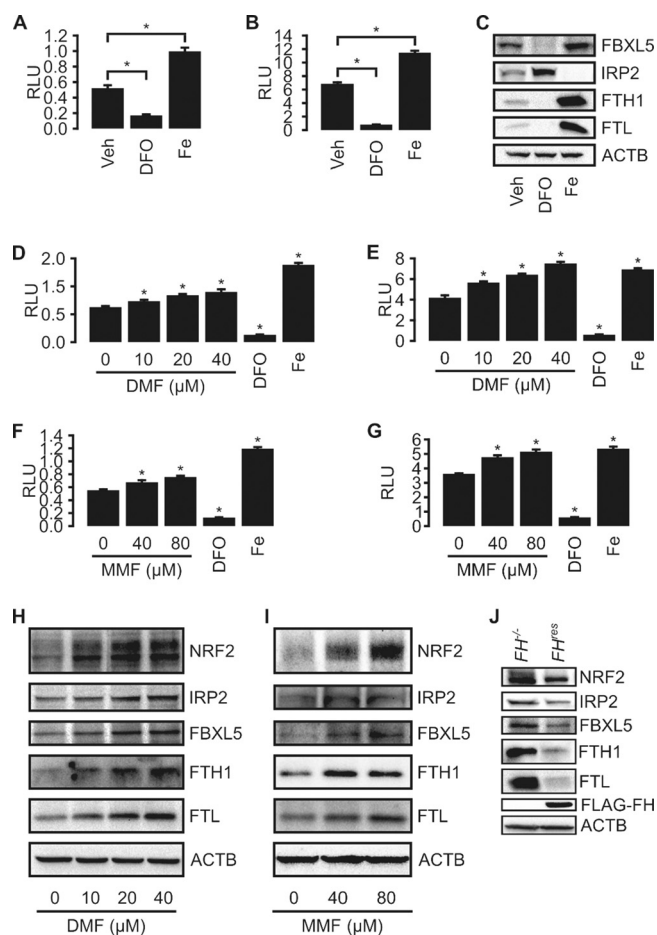
FIG 4 Fumarate inhibits IRP-mediated translational repression. (A and B) IRE reporter assays using the Dual-Glo luciferase assay (Promega) indicate appropriate responsiveness to iron levels for both pECE-FTL-IRE-LUX (A) and pECE-FTH1-IRE-LUX (B) cotransfected with pECE-RL into HEK293 cells. Cells were treated with ferric citrate (Fe; 200 micromolar) or an iron chelator (DFO; 200 micromolar) to modulate iron levels. Data are presented as means \pm standard deviations. * indicates a P value of <0.05 relative to vehicle (Veh) treatment, as determined by Student's t test. RLU, relative light units. (C) Immunoblots of HEK293 cells treated with DFO show increased IRP2 and decreased FTL, FTH1, and FBXL5 protein levels. Treatment with Fe resulted in opposite effects. ACTB was used as a loading control. (D to G) IRE reporter assays using the Dual-Glo luciferase assay (Promega) with dimethyl fumarate and monomethyl fumarate treatments. HEK293 cells were cotransfected with pECE-RL and either pECE-FTL-IRE-LUX (D and F) or pECE-FTH1-IRE-LUX (E and G). Cells were treated with increasing concentrations of either dimethyl fumarate (D and E) or monomethyl fumarate (F and G). Data are presented as means \pm standard deviations. * indicates a P value of <0.05 relative to vehicle treatment, as determined by Student's t test. (H and I) Western blots of HEK293 cells treated with increasing concentrations of DMF (H) or MMF (I) show dysregulated iron signaling, as indicated by simultaneously high protein levels of IRP2, FBXL5, FTL, and FTH1. ACTB was used as a loading control. (J) Western blots of UOK262- FH -/- control cells and UOK262- FH res cells. FH reconstitution leads to decreased NRF2, IRP2, FBXL5, FTH1, and FTL protein levels. ACTB was used as a loading control.
