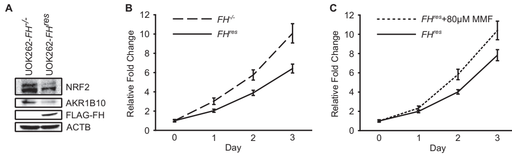
FIG 1 Fumarate accumulation confers chronic proliferation. (A) Western blots of NRF2 and its transcription target AKR1B10 after reintroduction of FH into the FH -/- HLRCC tumor cell line UOK262. \beta -Actin (ACTB) was used as a loading control. (B) Cell viability measured by formazan production in UOK262 cells ( FH -/- ) after reintroduction of FH (UOK262- FH res ). Data are presented as means \pm standard deviations of results from a representative experiment. Curves were statistically significantly different, as determined by two-way analysis of variance, for the FH genotype ( P < 0.001 ) but not for time ( P > 0.05 ). (C) Cell viability measured by formazan production in UOK262 cells ( FH -/- ) after reintroduction of FH (UOK262- FH res ) and 80 \mu M MMF treatment. Data are presented as means \pm standard deviations of results from a representative experiment. Curves were statistically significantly different, as determined by two-way analysis of variance, for MMF treatment ( P < 0.001 ) but not for time ( P > 0.05 ).
