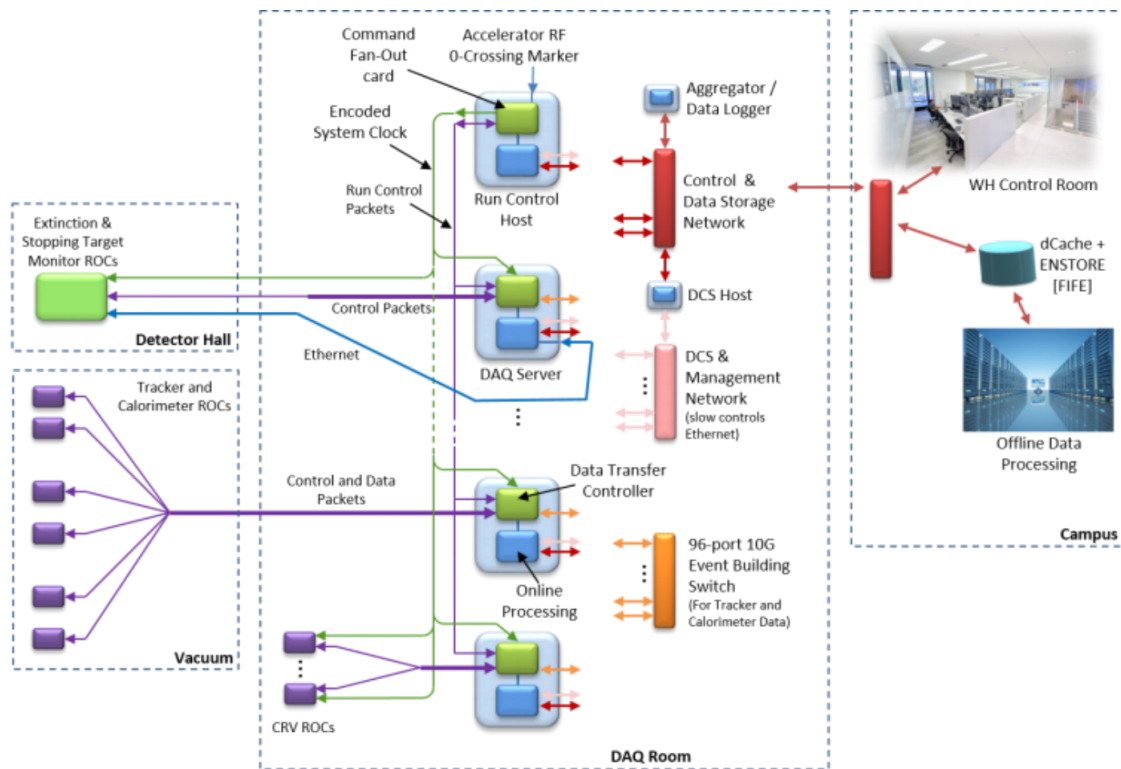
Figure 1. Mu2e TDAQ architecture and components diagram.
